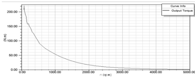
Figure 4. Output Torque and speed curve
