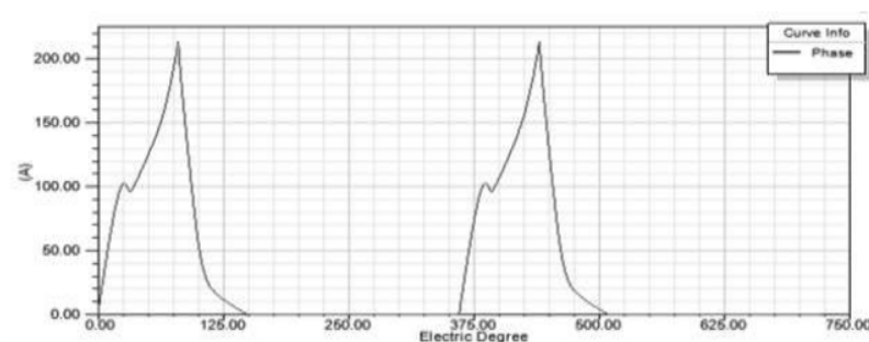
Figure 6. Rated phase current
