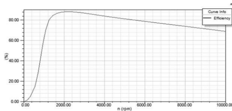
Figure 3. Efficiency to speed curve
