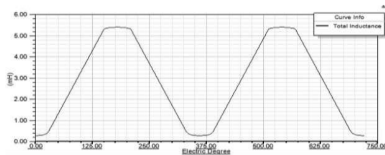
Figure 5. Air Gap inductance curve
