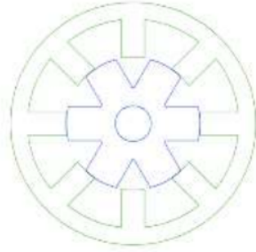
Figure 1. The proposed 8/6 switched reluctance motor
