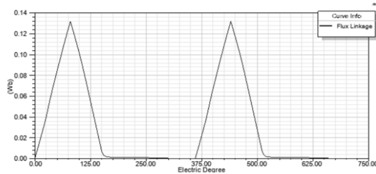
Figure 2. Flux linkage curve
