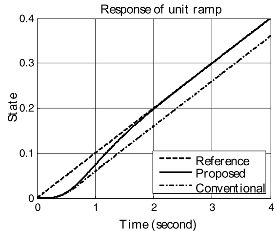
FIGURE 2. Integral state feedback for ramp input reference.
