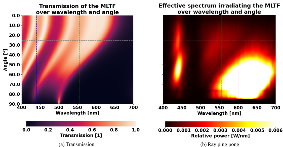
Figure 6. (a) Transmission of a multi-layer thin film that exhibits 28.9% more light compared to the reference design in forward direction. (b) The hypothetical, effective spectrum of light, which exits the conversion system and irradiates the multi-layer thin film. In both cases, the vertical dashed lines indicate the wavelengths contributing to the LED spectrum and the horizontal lines denote the separation between forward and non-forward direction.
