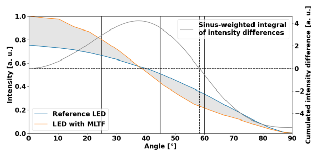
Figure 7. The normalized intensity of an LED with and without a multi-layer thin film (MLTF) is denoted on the left axis. The sinus-weighted integral over the intensity difference (grey area)—the so-called cumulated intensity difference —on the right axis indicates that a directionality increase can be achieved up to 58.4°. However, the peak of directionality increase is observed between 35° and 40°.
