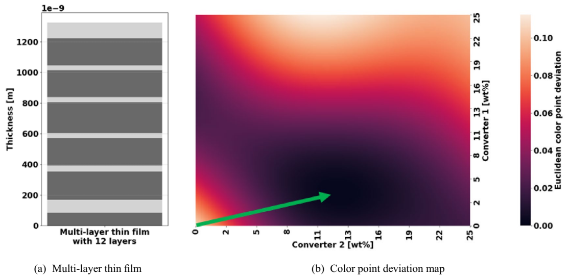
Figure 2. (a) Illustration of a multi-layer thin film consisting of two dielectric materials (TiO 2 in light grey and SiO 2 in dark grey). (b) The heatmap of the Euclidean color point deviation over weight percentages of two conversion materials for the multi-layer thin film in (a). The green arrow indicates the possible path of a local optimizer initialized near the origin of the search space to the optimal converter weight percentages.
