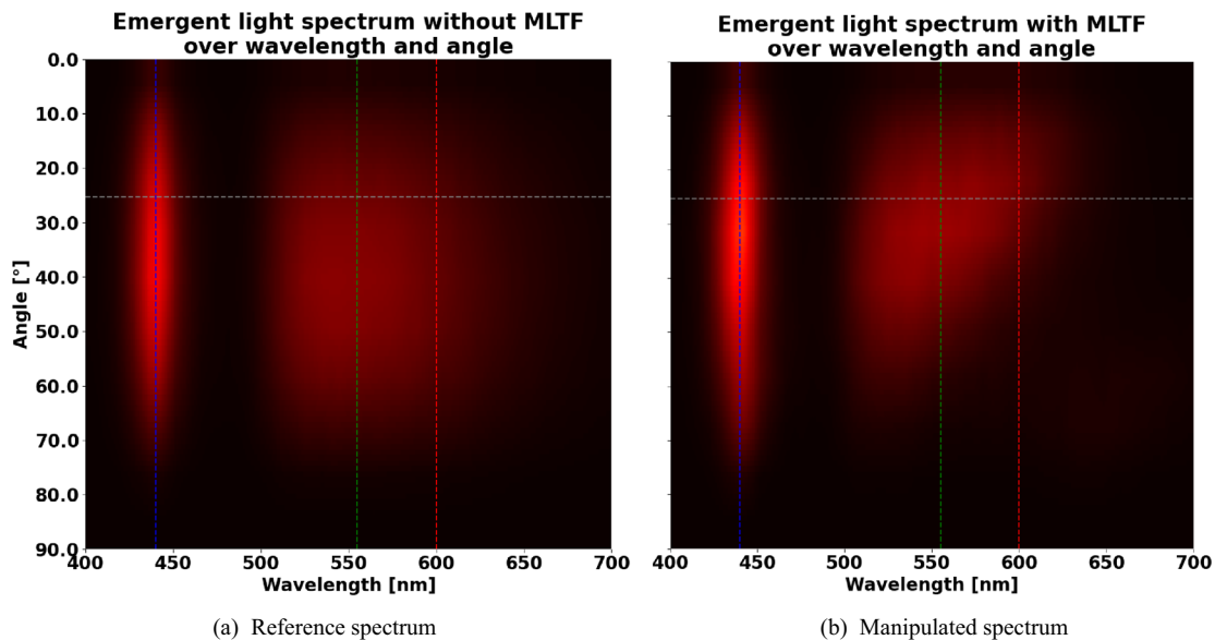
Figure 5. (a) Common angular and spectral distribution of relative power of a white LED without a multi-layer thin film. (b) Spectrum of a white LED with a multi-layer thin film that contains 28.9% more relative power compared to the reference design in forward direction. In each case, the blue chip wavelength (440 nm) and the green and red wavelengths (555 nm) and 600 nm) of the conversion materials are indicated by vertical dashed lines. The horizontal grey line indicates the \pm 25^\circ -forward direction. The color map for the heat maps coincides with Fig. 6.
