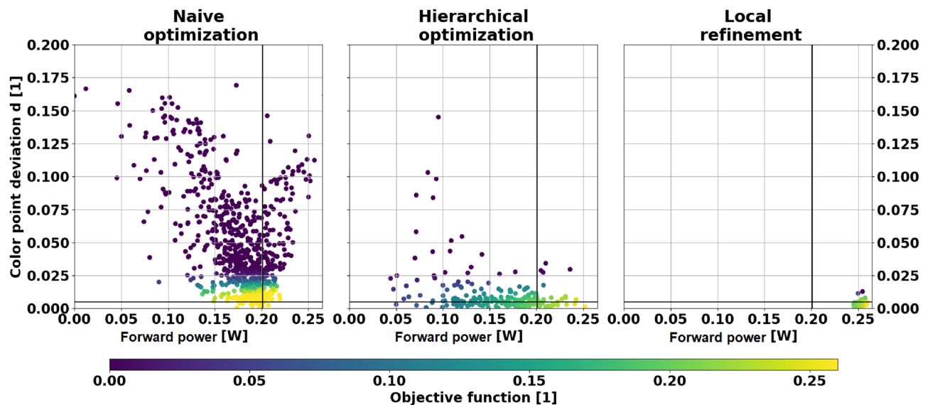
Figure 4. Color point deviation d^\alpha over power P^\alpha after joint (left, TS-EMO), hierarchical (middle, TS-SOO) and local (right, Downhill simplex) optimization for \alpha = 25^\circ . The horizontal black lines denote the color point deviation of 0.005 points, where W(0.005) = 0.99 holds. The vertical black lines denote the power of the reference design without multi-layer thin film. For each sample in these plots, the color map reflects the objective function values obtained by Eq. (2).
