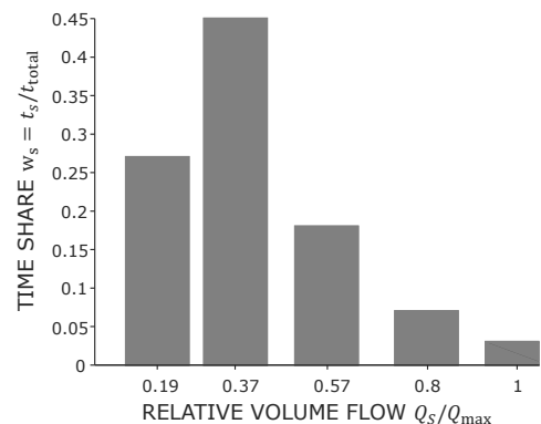
Figure 4: Time shares for different relative volume flows defining the reduced load profile for real booster stations according to [8] with the volume flow Q_s in load case s and the maximum volume flow Q_{max} .
