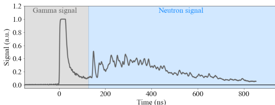
Figure 6. The raw nTOF detector trace recorded for a pitcher–catcher configuration located 7.2 m away with 27 cm lead shielding in front of the nTOF shows a gamma peak component followed by the neutron signal.
