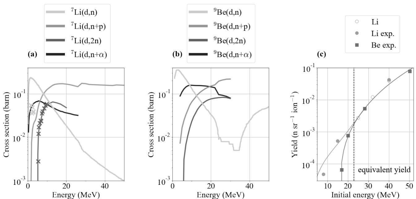
Figure 4. (a) Simulated neutron production cross sections (solid lines) [79–81] and corresponding experimental values (crosses) for lithium [82–84], (b) simulated neutron production cross sections for beryllium [79–81,85] and (c) experimental neutron yields (full circles) for lithium (8, 12, and 15 MeV from [86], 40 MeV from [87]) and for beryllium (squares) from [88] measured with a monoenergetic deuteron beam produced by an accelerator impinging on a thick converter target as well as simulation studies (empty circles) using Monte Carlo codes [89,90]. The plotted lines are a guide to the eye for the two different materials. To the right of the dashed line lithium and beryllium show equivalent neutron yield for incident deuterons with the same energy. (adapted from [76]).
