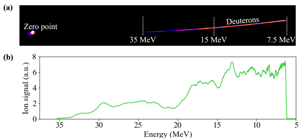
Figure 8. (a) Exemplary raw Thomson parabola trace of accelerated deuteron ion beam at 30° from target normal with integrated signal as a function of deuteron energy (b).
