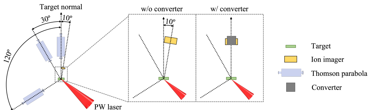
Figure 2. Ion beam diagnostics, three Thomson parabolas and an ion imager, placed around the converter during neutron generation, are set up at various angles from the target normal direction.
