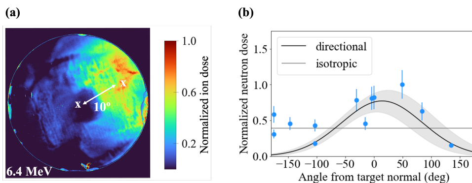
Figure 9. (a) Deuteron signal on first RCF layer within the converter at a depth equivalent to 6.4 MeV. (b) Neutron signal shown in bubble detector map in laser plane with two curves for the directional and isotropic neutron emission components to guide the eye.
