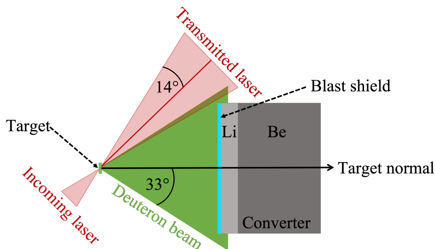
Figure 3. Top view of the setup (target size not to scale). The converter is placed in the target normal direction to capture the ion beam but outside the transmitted laser cone ( f/2 ) to avoid damages.
