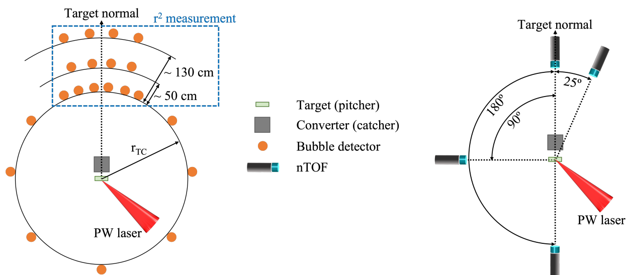
Figure 5. Setup for the neutron flux measurement in the laser plane using bubble detectors (left). The energy spectrum is measured using neutron time-of-flight detectors at selected angles (right).
