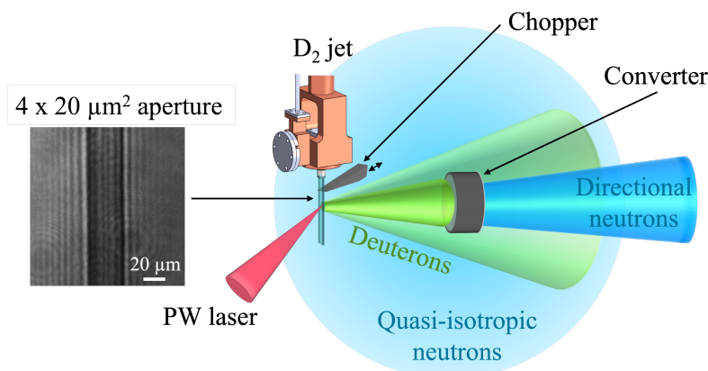
Figure 1. The platform setup consists of a petawatt laser, the cryogenic liquid D_2 jet target for deuteron acceleration, and the converter for neutron production. A shadowgraphy image of the planar cryogenic deuterium jet target is shown in the inset. The neutron beam has both a quasi-isotropic and a directional component.
