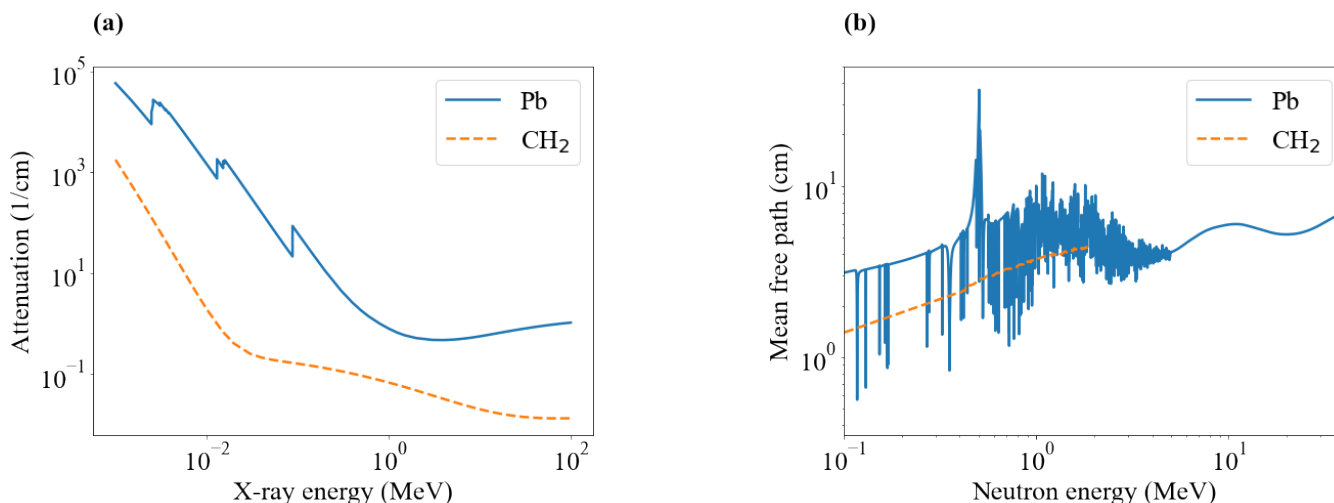
Figure 7. (a): X-ray attenuation coefficient (1/cm) shows superior x-ray attenuation up to three orders of magnitude in lead (Pb) over polyethylene (CH 2 ) [104]; (b): Neutron mean free path in lead and polyethylene [79,81,105,106].
