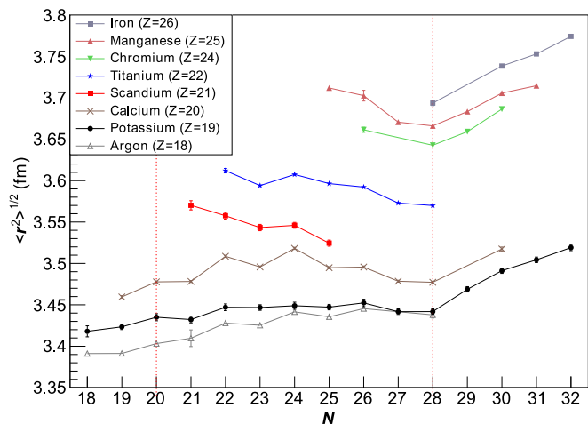
Fig. 7. (Color online.) Root mean square nuclear charge radii versus neutron number for the isotopes of Ar, K, Ca, Sc, Ti, Cr, Mn and Fe. Data for K results from this work.
