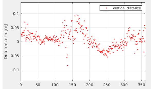
Figure 8. Height differences between vehicle based GNSS measurements (mode A) and DTM heights plus relative vehicle heights at the calibration track.
