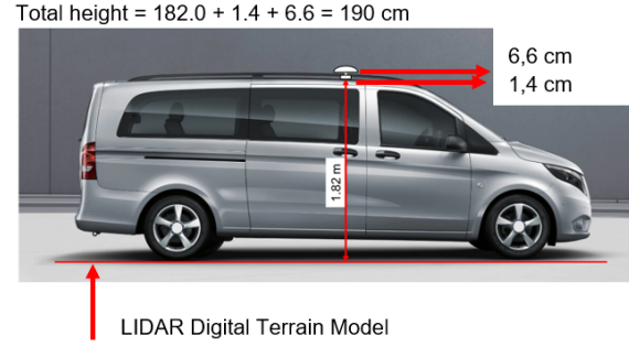
Figure 2. Precise absolute height information of GNSS antenna given a LIDAR DTM and the relative antenna height.
