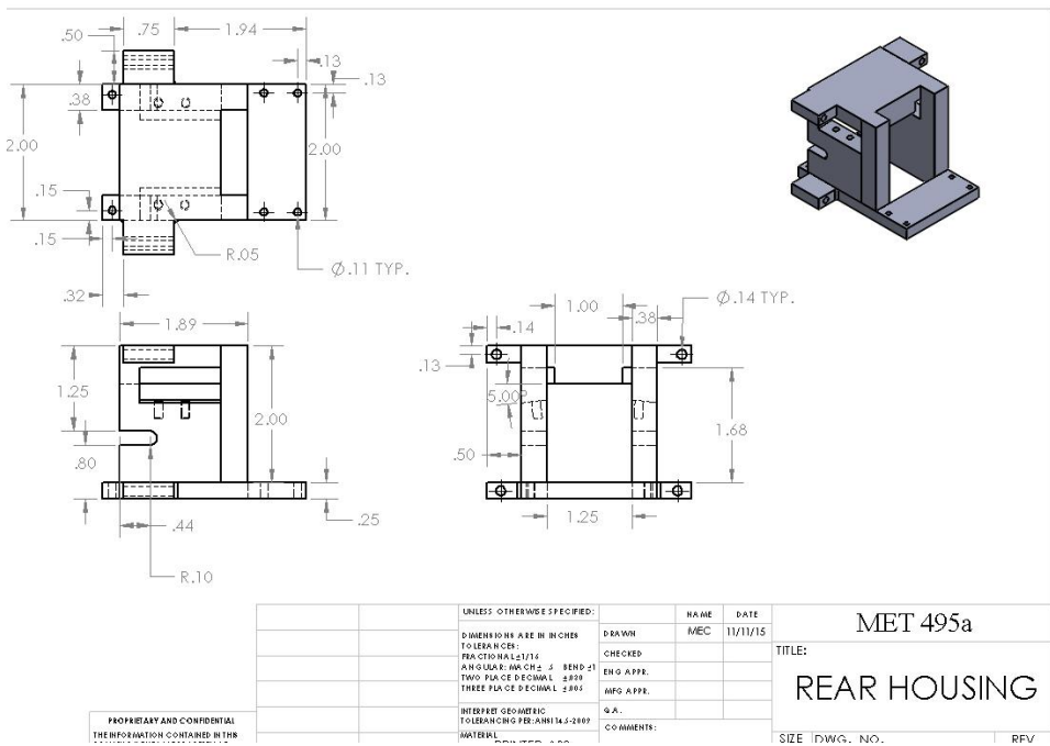
Figure 40 REAR ALLMOUNT/HOUSING
