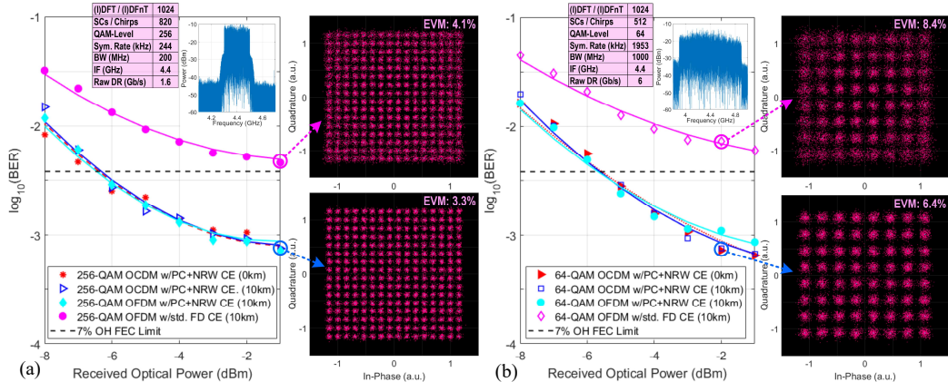
Fig. 2. ROP Vs. BER for 0 and 10 km with inset rx. constellations, IF spectra and numerology for 256 (a) and 64 (b) QAM OCDM/OFDM signals.
