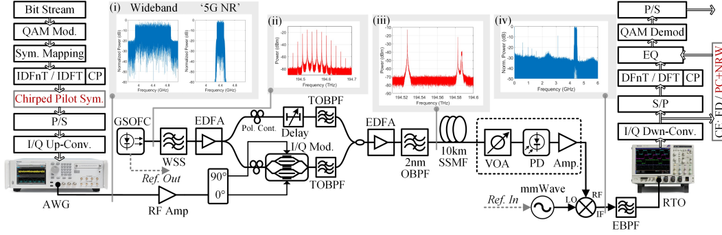
Fig. 1. Experimental optical/mm-wave system setup with electrical and optical spectra along the path shown in (i), (ii), (iii) and (iv).
