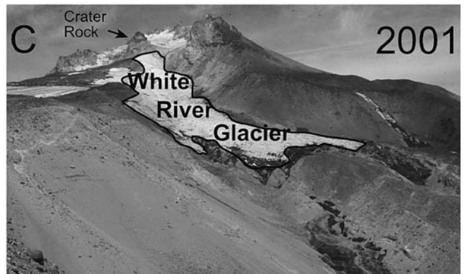
FIGURE 6. White River Glacier: (A) terminus changes, 1901–2001; (B) view of terminus from late Pleistocene and Holocene eruptive deposits in 1902 (Langille, 1903); and (C) same view and photo point on 14 September 2001. See photo point on Figure 6A. The dashed line at the top of the White River Glacier in 1902 indicates that the White River may have separated from the Coalman Glacier.
