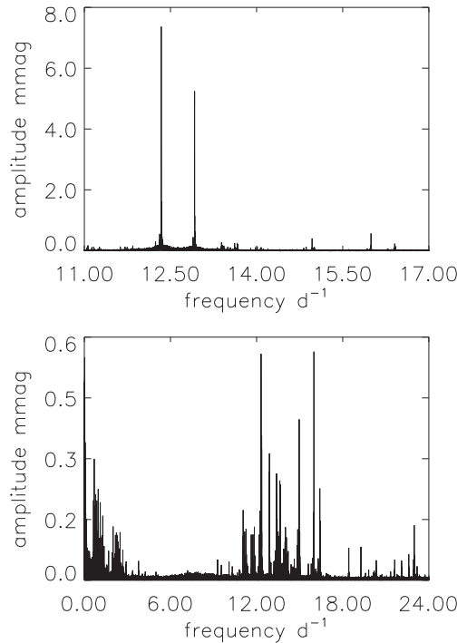
Figure 5. Top panel: The amplitude spectrum for the p-mode range of 11\text{--}17 \text{ d}^{-1} where most of the p-modes peaks are. The two high amplitude peaks, named \nu_1 and \nu_2 in the order of amplitude, are obvious. Bottom: The full frequency range after pre-whitening by \nu_1 and \nu_2 where a plethora of peaks can be seen.
