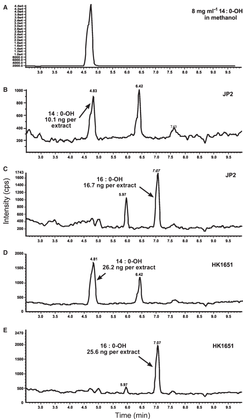
Figure 5. Identification of hydroxylated myristic and palmitic acids in leukotoxin A (LtxA) extracts from Aggregatibacter actinomycetemcomitans , strains JP2 and HK1651. Extracted ion chromatograms showing the multiple reaction monitoring (MRM) of [M^+CH_3COO]^- \rightarrow [M-H]^- for C14:0-OH (303.2/243.2 amu transition) and C16:0-OH (331.2/271.2 amu transition). The C14:0-OH standard was injected onto a reversed phase, Zorbax® Eclipse XDB-C18, 2.1 × 50 mm, 1.8 μm column to optimize the liquid chromatography and MRM conditions for measurement. The MRM method was subsequently expanded to monitor C16:0-OH. Dried samples of JP2 and HK1651 LtxA were then reconstituted in 1.0 ml HPLC-grade methanol and injected along with a calibration curve for C14:0-OH ranging
