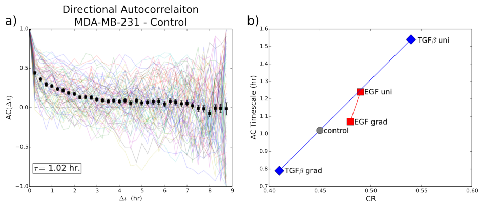
Fig. 3.3. a) Directional Autocorrelation from control dataset. Light-colored trajectories indicate autocorrelations for individual cell trajectories. Timescale \tau is calculated using Eq. 3.4. b) Directional autocorrelation timescales and CR values for all experimental assays. Data points are color-coded based on chemical environment.
