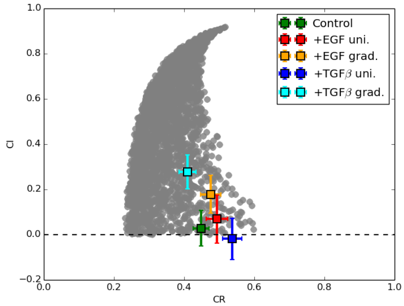
Fig. 3.6. Theoretical bounds on chemotactic performance based on the biased persistent random walk model. Gray dots represent possible theoretical CI and CR values for a BPRW. Colored squares are experimentally recorded values for different environmental conditions.
