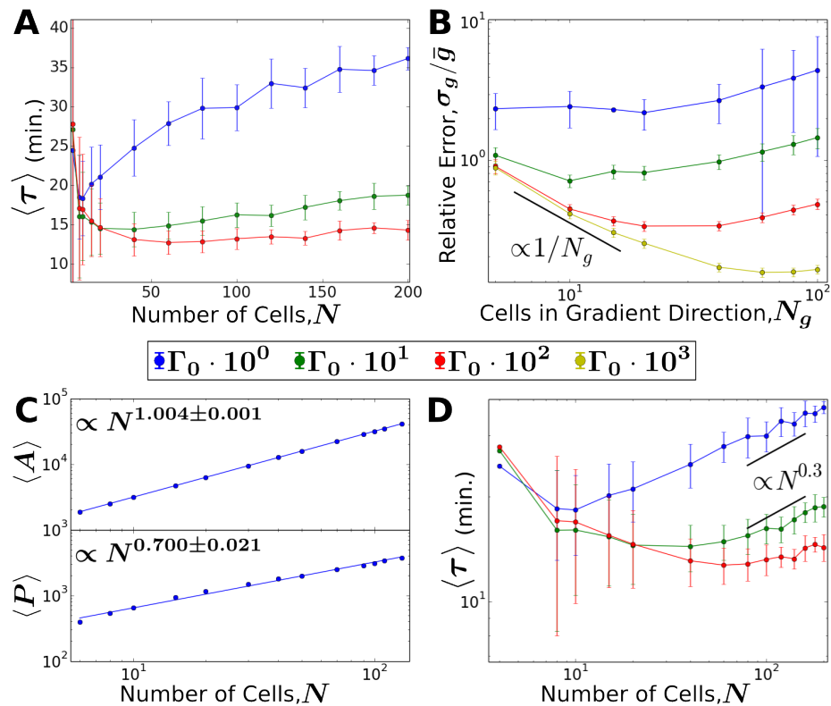
Fig. 5.3. Tradeoff between sensing and drag leads to a minimum mean first-passage time (MFPT) with cluster size. \Gamma_0 = 0.80 (\mu\text{m min})^{-1} . (A) MFPT for various values of the exchange rate per unit contact-length \Gamma . (B) Relative error in gradient sensing for various values of \Gamma . (C) Area A and perimeter P scaling relationships with the number of cells N in a cluster. (D) MFPT results in A on a log-log scale, compared with the geometric prediction arising from C. All error bars represent standard deviation.
