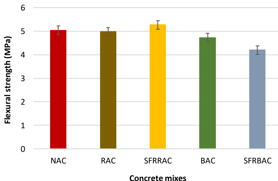
Figure 4.8: Flexural strength of concrete for different mixes at 28 days.
