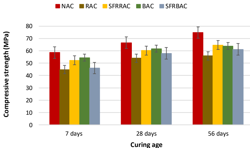
Figure 4.3: Effect of curing age on the compressive strength of concrete for different mixes.
