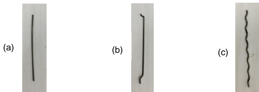
Figure 3.11: 60mm steel fibres: (a) Straight (b) Hooked-ended (c) Undulated.
