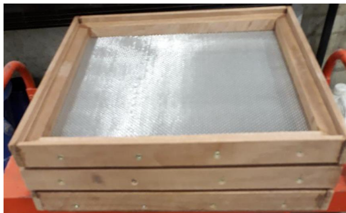
Figure 3.5: A set of wire mesh for grading of fine aggregates.
