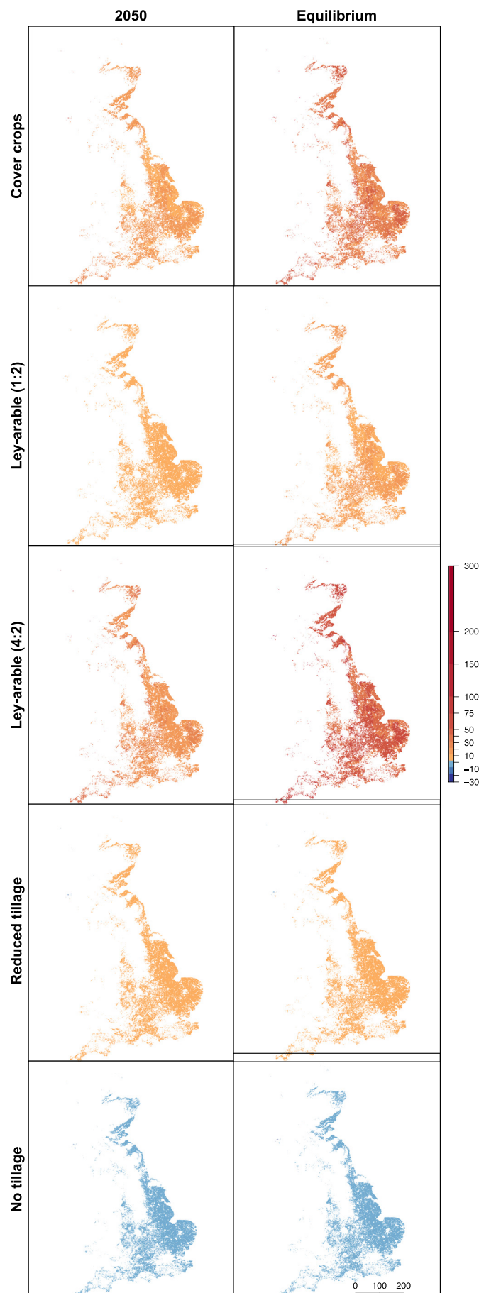
Fig. 3. Great Britain arable soil organic carbon (SOC) stocks ( \text{t}\cdot\text{ha}^{-1} ) at 1 \text{ km}^2 resolution. Colour indicates difference from baseline (0–30 cm), following implementation of cover crops, ley-arable rotations and reduced tillage intensity after 30 years and once a new equilibrium is reached. The two scenarios for ley-arable rotations are one year ley-phase and two years arable cropping (L1A2), and four years ley-phase and two years arable cropping (L4A2). 1 \text{ km}^2 resolution for arable land in Great Britain identified using the CEH land cover map (Rowland et al., 2017). Scale bar in km.
