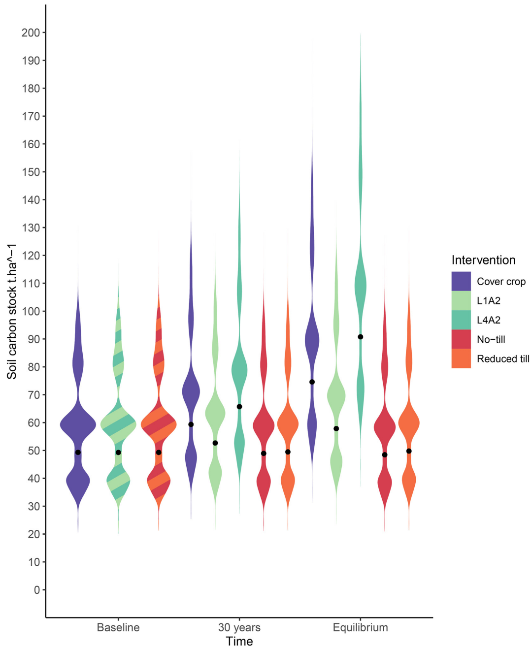
Fig. 2. Distribution of Great Britain arable soil organic carbon (SOC) stocks ( \text{t}\cdot\text{ha}^{-1} ). Baseline (assumed current, using WISE30sec values) (Batjes, 2016) and following implementation of cover crops, ley-arable rotations and reduced tillage intensity after 30 years (i.e. around the year 2050) and once a new equilibrium is reached, to 30 cm depth. Violin plots show distribution of mean values from each 1\text{ km}^2 model run for in Great Britain. Two ley-arable systems are modelled: L1A2, one year ley-phase and two years arable cropping, and L4A2, four years ley-phase and two years arable cropping. Simulations for two ley-arable scenarios and two reduced tillage scenarios were run together, respectively, hence shared baselines.
