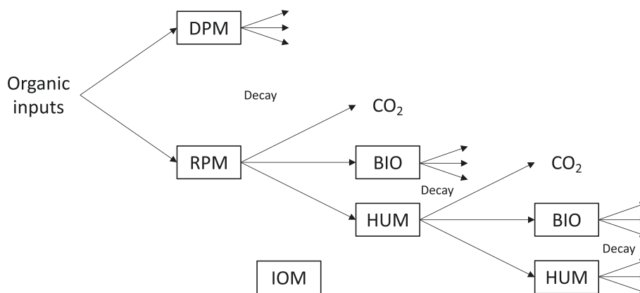
Fig. 1. Conceptual soil carbon pools in RothC-26.3. DPM: decomposable plant material, RPM: resistant plant material, BIO: microbial biomass, HUM: humified organic matter, IOM: inert organic matter, after Coleman and Jenkinson (2014). Decay of pools determined by first-order kinetics with decomposition rate constant, apart from small inert pool resistant to decomposition.
