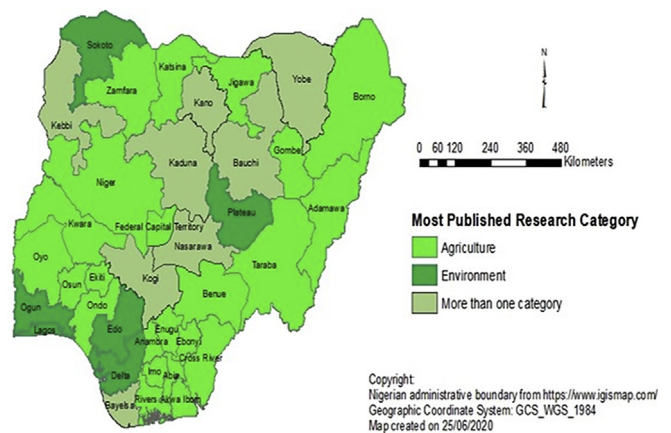
Figure 4. Most published research categories on CC impacts in Nigeria (1962–2019).
