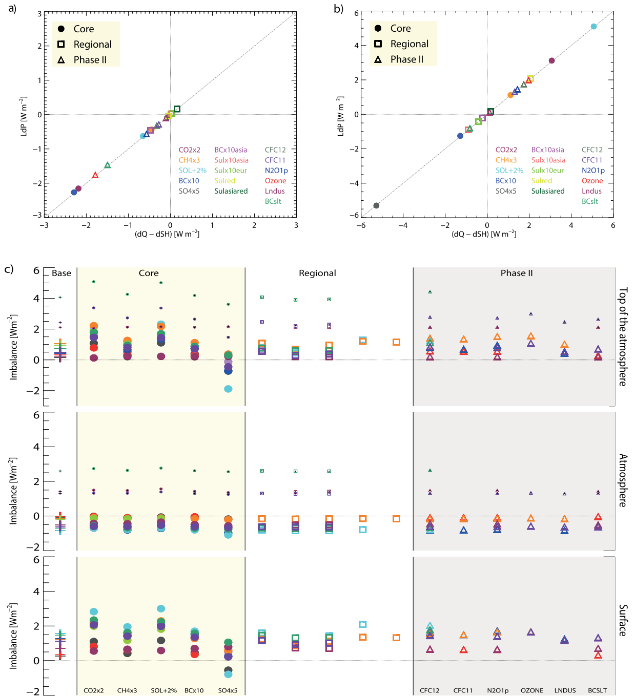
Fig. 2 The PDRMIP multi-model mean of precipitation in energy fluxes ( W m^{-2} ) is shown as a function of change in the atmospheric radiative cooling and the reduction of surface sensible heat for all PDRMIP experiments in the fsst simulations (a) and coupled simulations (b). The TOA, atmospheric and surface imbalance in the Base and PDRMIP perturbation experiments (c). Radiative imbalance at top of the atmosphere, in the atmosphere and at the surface for all PDRMIP experiments and models in the coupled atmosphere and ocean simulations. Small symbols are included for reported values for three of the models whereas regular symbols take into account difference between the top model layer and TOA.
