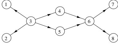
Figure 3: A Citation Graph (A Counterexample)
