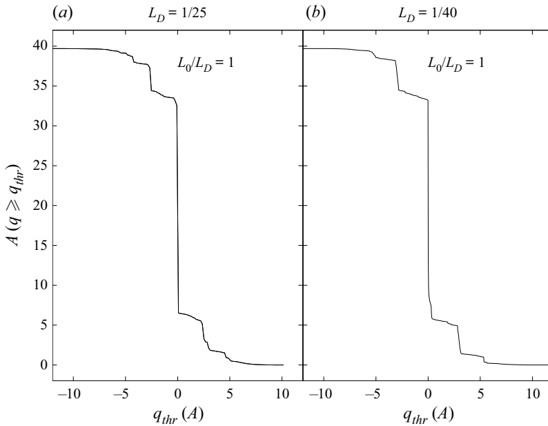
Figure 8. Potential vorticity staircases for simulations with L_D = 1/25 , L_0/L_D = 1 (a, t = 200\,000 ) and L_D = 1/40 , L_0/L_D = 1 (b, t = 604\,500 ). The structures are the same, suggesting the staircase structure depends only on the ratio L_0/L_D .
