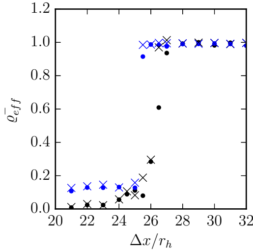
Figure 7. Merger efficiency for the central anticyclones \bar{\varrho}_{eff}^{-} = (V_{tot}^{-} - V_{max}^{-})/V_{max}^{-} at t = 200 , for \Delta z/r_h = 0 (black) and \Delta z/r_h = 1.25 (blue). \bullet : asymmetric baroclinic tripolar eddies, \times : symmetric baroclinic tripolar eddies (Colour online).
