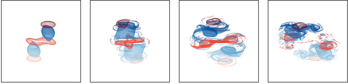
Figure 23. Evolution of the vortex bounding contours for two symmetric, isolated baroclinic, tripolar eddies for \Delta z/r_h = 2.5 and \Delta x/r_h = 2.1 at, from left to right, t = 3, 14, 22.5 and 34.5 . The contours are viewed orthographically at an angle of 65^\circ from the vertical axis. The colour shading indicates the depth z of the contours, with lighter contours near the bottom. Red contours bound positive (cyclonic) PV, blue contours bound negative (anticyclonic) PV (Colour online).
