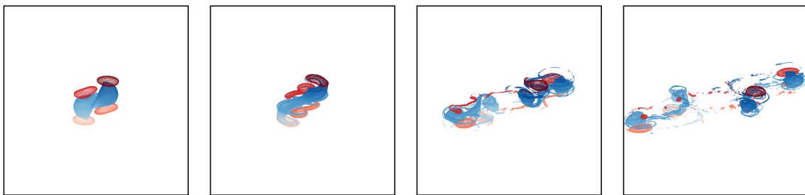
Figure 22. Evolution of the vortex bounding contours for two symmetric, isolated baroclinic, tripolar eddies for \Delta z/r_h = 1.25 and \Delta x/r_h = 2.2 at, from left to right, t = 2, 5.5, 20 and 30 . The contours are viewed orthographically at an angle of 65^\circ from the vertical axis. The colour shading indicates the depth z of the contours, with lighter contours near the bottom. Red contours bound positive (cyclonic) PV, blue contours bound negative (anticyclonic) PV (Colour online).
