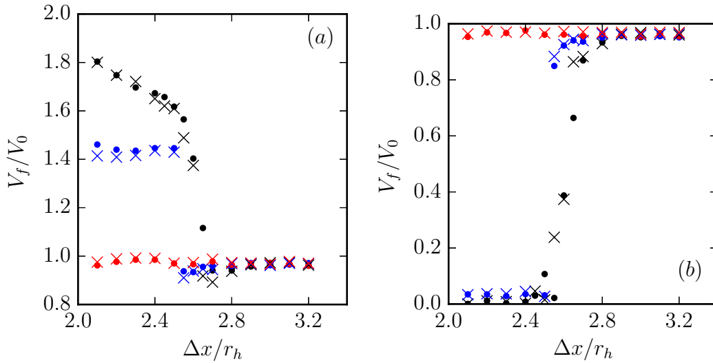
Figure 4. (a) Ratio of the volume at t = 200 V_f to the initial volume V_0 , of the largest (anticyclonic) vortex present in the flow vs \Delta x/r_h for the asymmetric configuration ( \bullet ) and symmetric configuration ( \times ) for \Delta z = 0 (black), \Delta z/r_h = 1.25 (blue) and \Delta z = 2.5 (red). (b) V_f/V_0 for the second largest anticyclone (same conventions). (Colour online).
