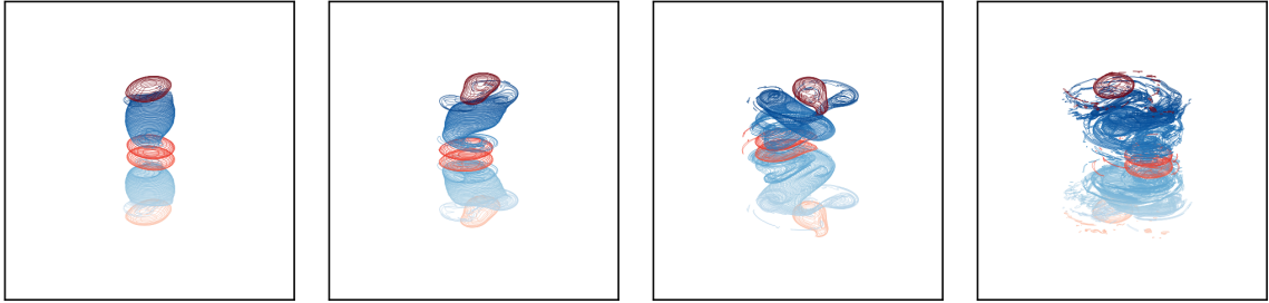
Figure 24. Evolution of the vortex bounding contours for two symmetric, isolated baroclinic, tripolar eddies for \Delta z/r_h = 3 and \Delta x/r_h = 0 at, from left to right, t = 15.5, 20.5, 27.5 and 44 . The contours are viewed orthographically at an angle of 65^\circ from the vertical axis. The colour shading indicates the depth z of the contours, with lighter contours near the bottom. Red contours bound positive (cyclonic) PV, blue contours bound negative (anticyclonic) PV (Colour online).
