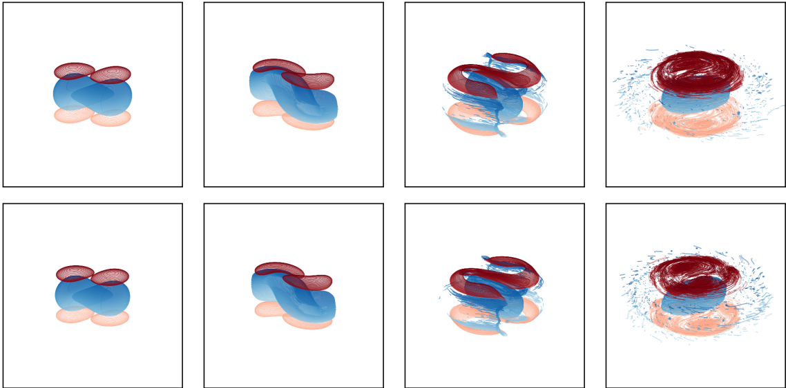
Figure 5. Evolution of the vortex bounding contours for two interacting baroclinic, tripolar eddies for \Delta x/r_h = 2.1 , and from left to right at t = 1, 3, 10, and 200 . First row: \Delta z = 0 and the eddies are asymmetric. Second row: \Delta z = 0 , and the eddies are symmetric. The contours are viewed orthographically at an angle of 65^\circ from the vertical axis. The colour shading indicates the depth z of the contours, with lighter contours near the bottom. Red contours bound positive (cyclonic) PV, blue contours bound negative (anticyclonic) PV (Colour online).
