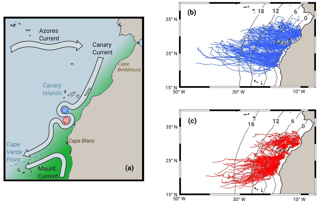
Figure 2. (a) Schematic of the formation mechanism of nearshore-generated CEs and AEs by meandering of the coastal Canary current and of the regional system of currents; color shading illustrates the mean regional pattern of tracers such as DIN and PON, with green representing higher concentrations. Tracks of long-living eddies (>6 months) for (b) CEs and (c) AEs in the northern CanUS plotted until their 18th month of life, and showing the north-west drift of CEs and south-west drift of AEs. Isolines in subplots (b) and (c) indicate the mean age of eddies (in months) at each offshore distance.
