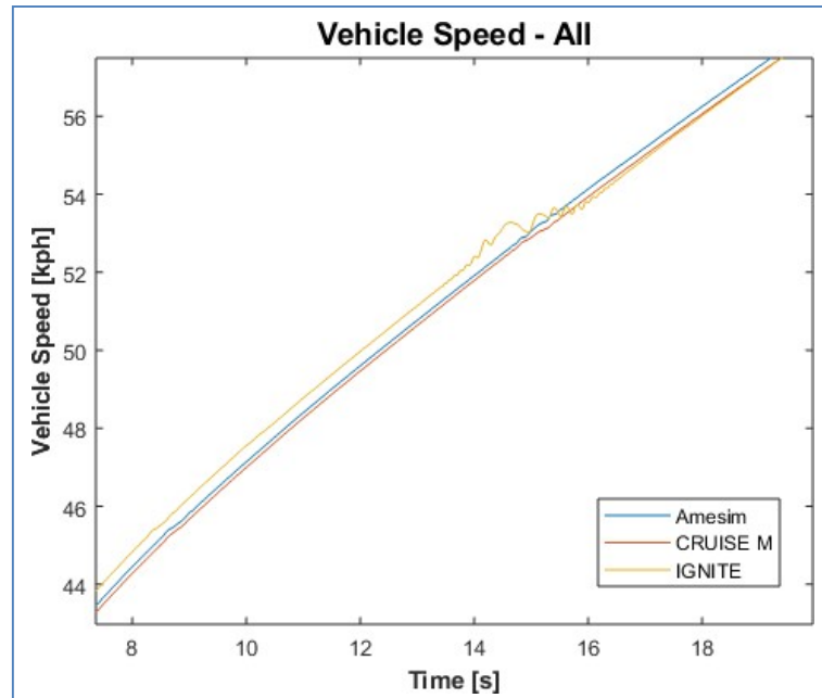
Figure 8 Detailed Vehicle Speed Comparison
