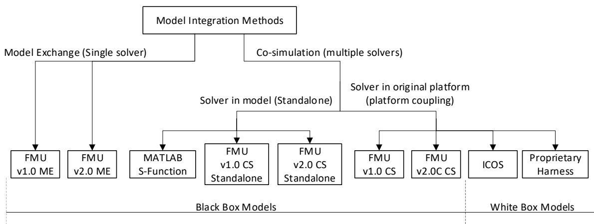
Figure 1 Tree diagram of model integration methods most commonly used in automotive applications
