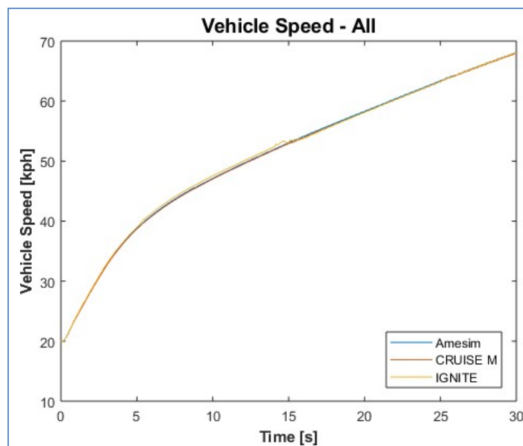
Figure 7 Vehicle speed vs. Time plot of the simulated MME-Vehicle combinations
