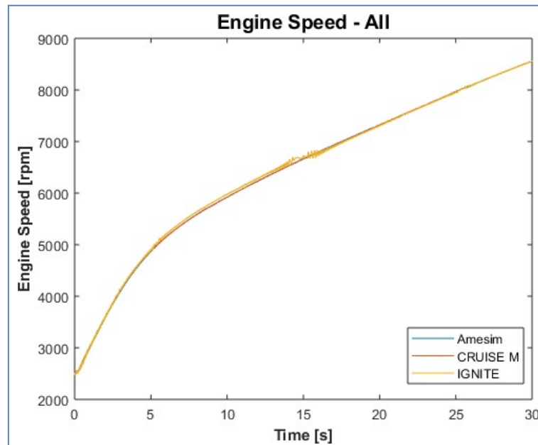
Figure 6 Engine speed vs. Time plot of the simulated MME-Vehicle combinations
