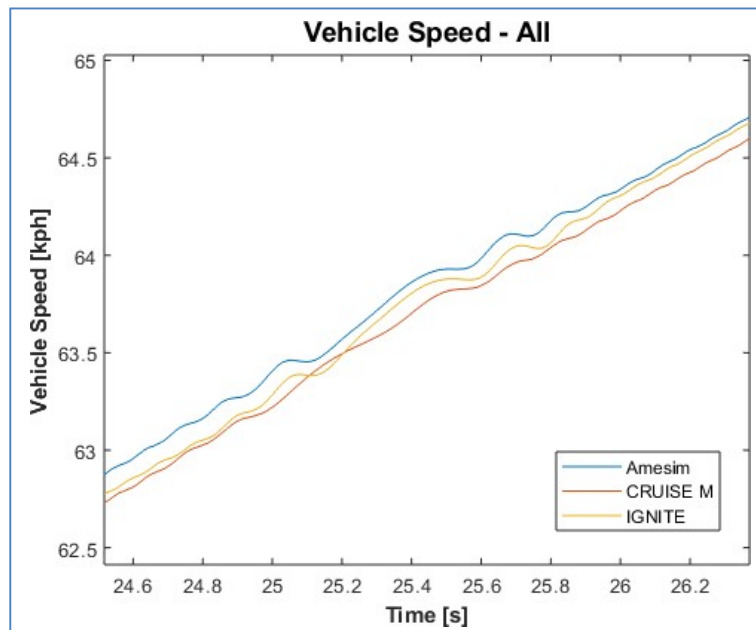
Figure 9 Detailed Vehicle Speed Comparison (2)
