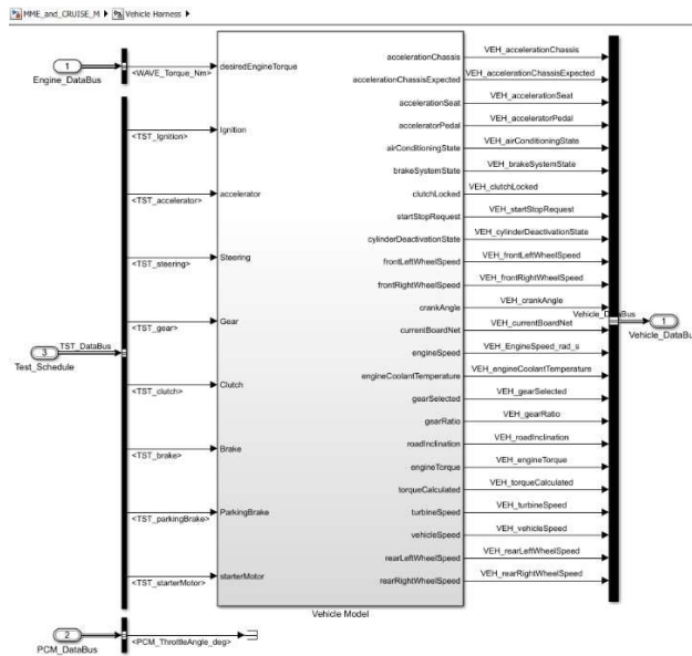
Figure 5 Content of the "Vehicle Harness" block
