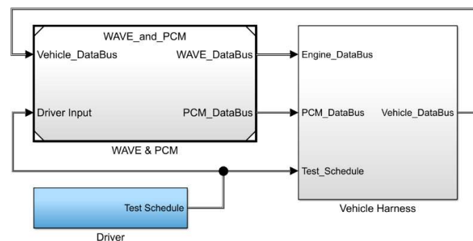
Figure 3 Top-level Simulink block diagram of the MME
