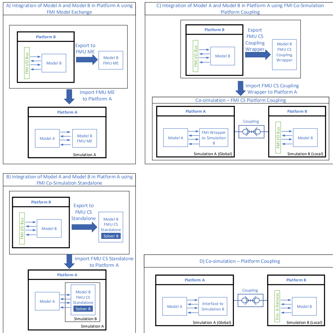
Figure 2 Diagrams of model FMU and dedicated harness model integration
