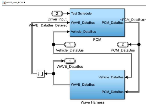
Figure 4 Block diagram of the "WAVE_and_PCM" model
