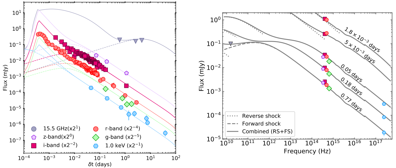
Figure 6. Left: The radio to X-ray light curves of the GRB 180418A afterglow and the best-fit RS+FS model (solid lines) with a magnetization parameter of R_B \approx 5.2 and an initial jet Lorentz factor of \Gamma_0 \approx 150 . For each band, the FS component is indicated with dashed lines. Right: Radio to X-ray spectral energy distribution of the GRB 180418A afterglow spanning 1.8 \times 10^{-3} days to 0.77 days after the burst, together with the best-fit model (solid lines) decomposed into reverse (dotted) and forward shock (dashed) components. The radio upper limit constrains the peak flux and frequency of the FS spectrum, necessitating an RS component in the optical before \approx 0.05 days.
