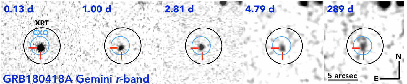
Figure 4. Gemini-North and South GMOS r -band imaging sequence of the optical afterglow of GRB 180418A, over \delta t = 0.13 - 4.79 days. A deep, template image at \delta t \approx 289 days (last panel) reveals a faint, underlying host galaxy with r = 25.69 \pm 0.21 mag. The position of the optical afterglow (red cross-hairs) is coincident with the Chandra (CXO) position ( 3\sigma radius including astrometric uncertainty; blue circle) and the enhanced XRT position ( 3\sigma radius; black circle). The scale and orientation of the images is denoted in the last panel, and the last two panels have been smoothed for display purposes.
