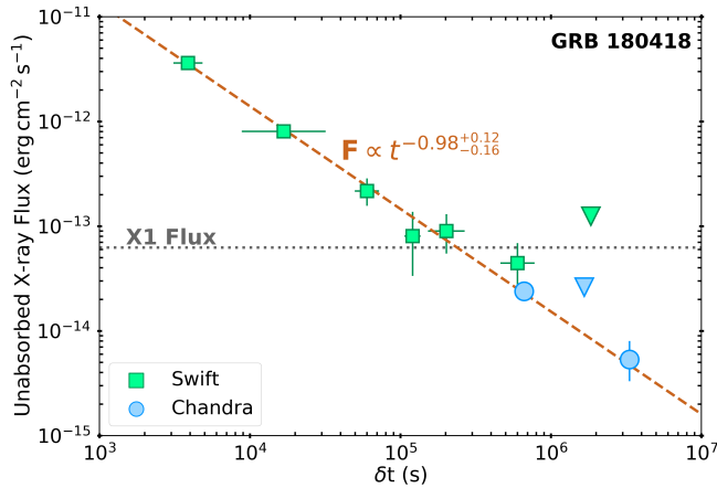
Figure 3. The Swift /XRT (green squares) and Chandra /ACIS-S (blue circles) unabsorbed X-ray flux light curve (0.3–10 keV) for GRB 180418A. Each observation is log-centred with the time errors denoting the duration of each observation. The flux errors are 1\sigma . In some cases, the symbols are bigger than the errors. The Swift and Chandra 3\sigma upper limits are indicated with green and blue arrows, respectively. The dashed light brown line represents the best-fit single power-law model with \alpha_X = -0.98_{-0.16}^{+0.12} . The dotted horizontal grey line shows the unabsorbed X-ray flux level of X1, \sim 6.24 \times 10^{-14} erg cm ^{-2} s ^{-1} (see Table 1).
