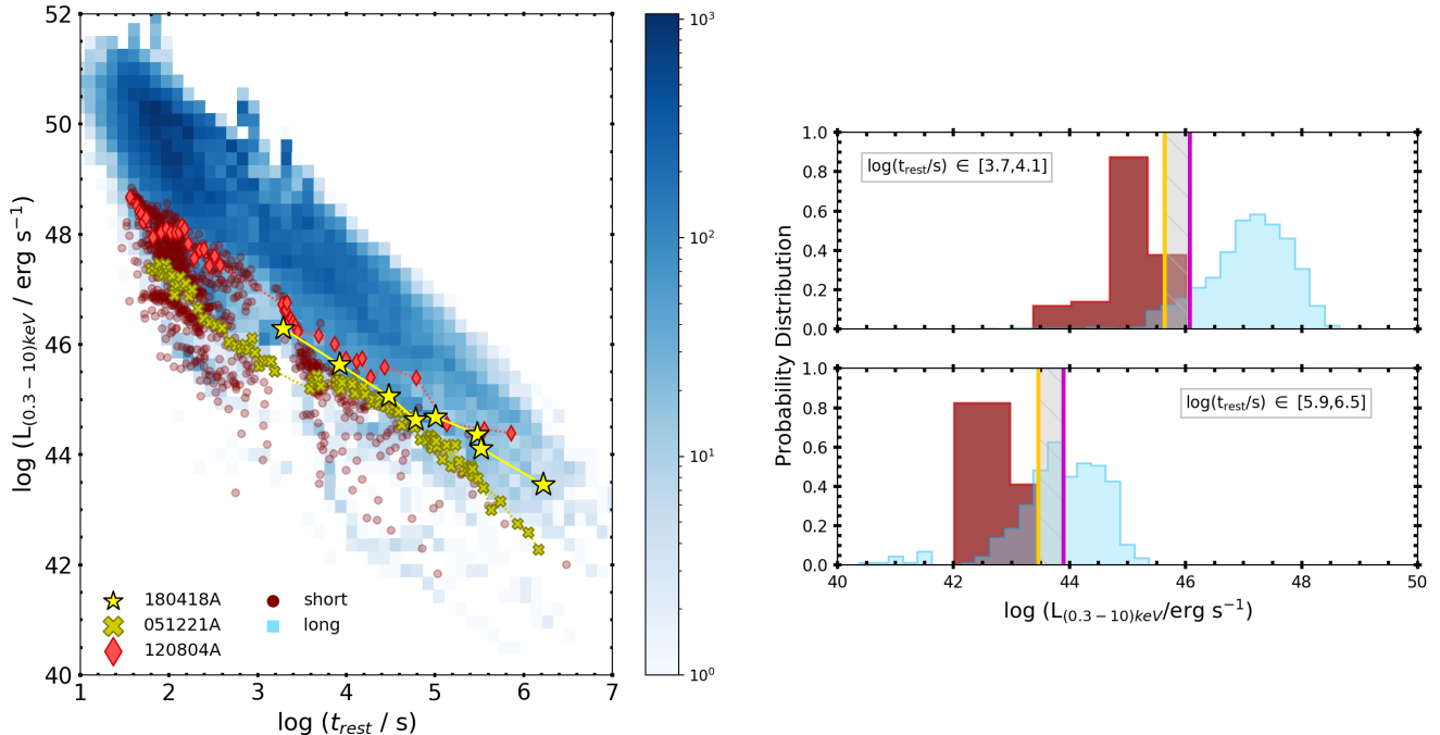
Figure 7. Left: The X-ray luminosity (0.3 – 10.0 keV) versus rest-frame time plot of all the GRBs detected by Swift /BAT with known redshifts. The long GRB population ( T_{90} > 2 s) is shown in blue, where the different shades in color represents the density of available data. The short GRB population ( T_{90} \leq 2 s) is represented by deep red circles. For plotting purposes, we only show the X-ray luminosity light curve of GRB 180418A at z = 1 (yellow stars). Those short GRBs that display similar X-ray behavior to GRB 180418A (Section 5) are shown with different point markers (yellow x’s and red diamonds). Right: Distribution of the X-ray luminosity (0.3 – 10.0 keV) for the short (red) and long (blue) GRB populations at \log(\delta t_{\text{rest}}/s) \approx 4 (top panel) and \log(\delta t_{\text{rest}}/s) \approx 6 (bottom panel). The grey shaded area indicates the potential X-ray luminosity values for the GRB 180418A afterglow since the redshift estimate ranges between z = 1 and z = 1.5 (see Section 4.1). The X-ray luminosity of the afterglow at z = 1 is shown with dark yellow vertical lines, while the dark pink vertical lines indicate the luminosity at z = 1.5 .
