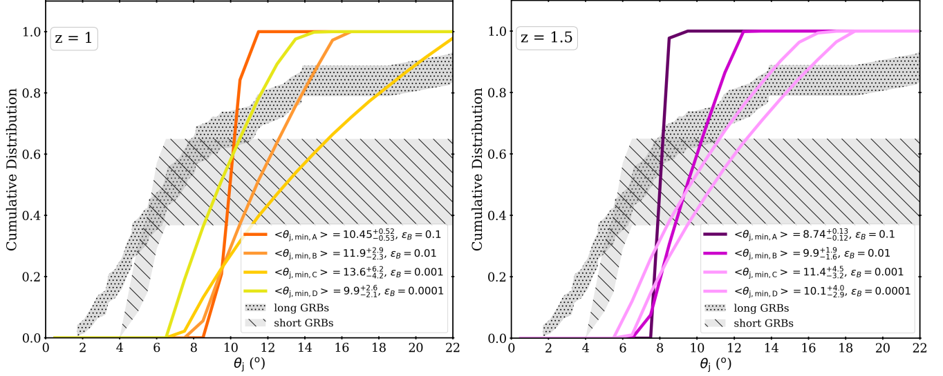
Figure 9. The cumulative distributions of the minimum values of the jet opening angles ( \theta_j ) at z = 1 (left) and z = 1.5 (right) for GRB 180418A. The different colors correspond to the different cases shown in Table 3. The cumulative distributions of the opening angles for short and long GRBs are shown in the dashed light-grey and dotted dark-grey areas, respectively. In this case, we have applied survival statistics for right-censored data to account for the lower limits of the opening angles in both populations. The plotted areas correspond to their 68% confidence intervals.
