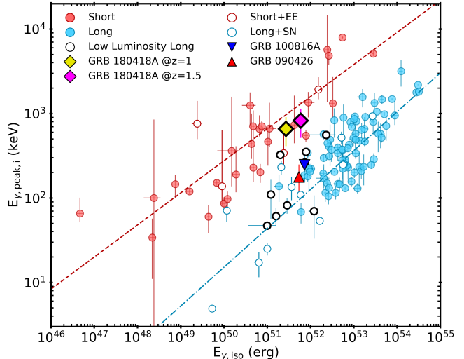
Figure 8. The E_{\gamma,\text{peak},i} - E_{\gamma,\text{iso}} relation for Swift and Fermi short (light red circles) and long (blue circles) GRBs (Minaev & Pozanenko 2020), along with GRB 180418A (diamonds) at z = 1 and z = 1.5 . We highlight short GRBs with extended emission (red open circles), and long GRBs with detected supernovae (blue open circles). GRB 180418A is fully consistent with the short GRB population in the E_{\gamma,\text{peak},i} - E_{\gamma,\text{iso}} plane and is a clear outlier compared to the space occupied by long GRBs (and the Amati correlation). Best-fit correlation models are indicated with lines (red dashed line for short GRBs and blue dashed-dotted line for long GRBs; Minaev & Pozanenko 2020). We also highlight the ambiguous cases of GRBs 090426 (red triangle; Antonelli et al. 2009) and 100816A (blue triangle; D’Avanzo et al. 2014, see Section 6.1), and the low luminosity long GRBs (circles with black borders; Dereli et al. 2017).
