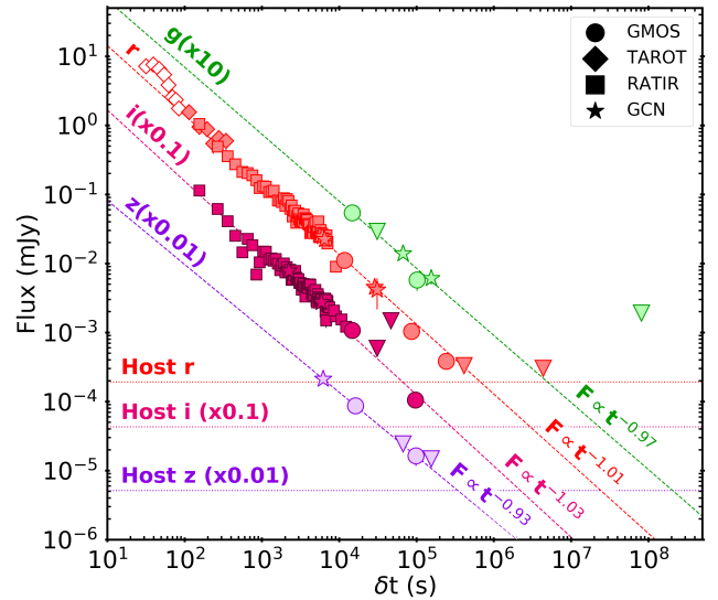
Figure 5. Optical afterglow light curves of GRB 180418A in the griz filters. Circles represent our new Gemini afterglow data (Table 2), r -band upper limits indicate 3\sigma upper limits (red triangles). Literature data from TAROT (diamonds), RATIR (squares) and other sources (stars) together with upper limits (triangles) are also shown (Becerra et al. 2019; Choi et al. 2018; Guidorzi et al. 2018; Horiuchi et al. 2018; Malesani et al. 2018; Misra et al. 2018; Schady 2018; Schady & Chen 2018; Sota et al. 2018; Xin et al. 2018). Only those observations in the riz filters for which the host galaxy contribution is less than 5% of the total optical flux are plotted. Observations which are ignored in the power-law fit are shown as open symbols. Horizontal lines denote the flux of the host galaxy, while dashed lines indicate the best-fit power-law decay models for the different bands.
