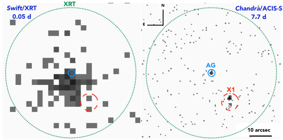
Figure 2. X-ray imaging of the Swift /XRT (left) and Chandra /ACIS-S (right) images of GRB 180418A in the 0.5–8 keV energy bands. The large dotted green circle indicates the XRT source subtraction region while the blue circle shows the 3\sigma source region from the Chandra observation. The small dashed red region in both images shows X1, which adds an extra contribution to the count rate extracted from the XRT source region.
