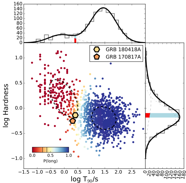
Figure 1. The Hardness- T_{90} plane of 1405 bursts detected by Fermi /GBM (Bhat et al. 2016). The color scale from red to blue indicates the probability that a given event is a long GRB ( P_{\text{long}} ), where a value of P_{\text{long}} = 0 indicates a short GRB. In the projected histograms for each parameter (top and right), the contributions from the short (red) and long (light blue) GRB populations at the position of GRB 180418A are shown, containing the classification based only on either duration or hardness alone. We use two-dimensional Gaussians to fit the distributions, where dashed-line ellipses correspond to 1\sigma confidence. The hexagon and pentagon indicate the locations of GRB 180418A and GRB 170817A, respectively. The position of each source has also been indicated with black lines in the probability color bar.
