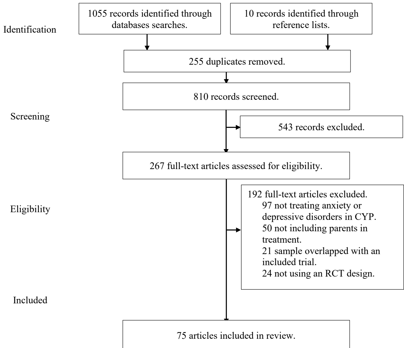
Figure 1 Study selection
