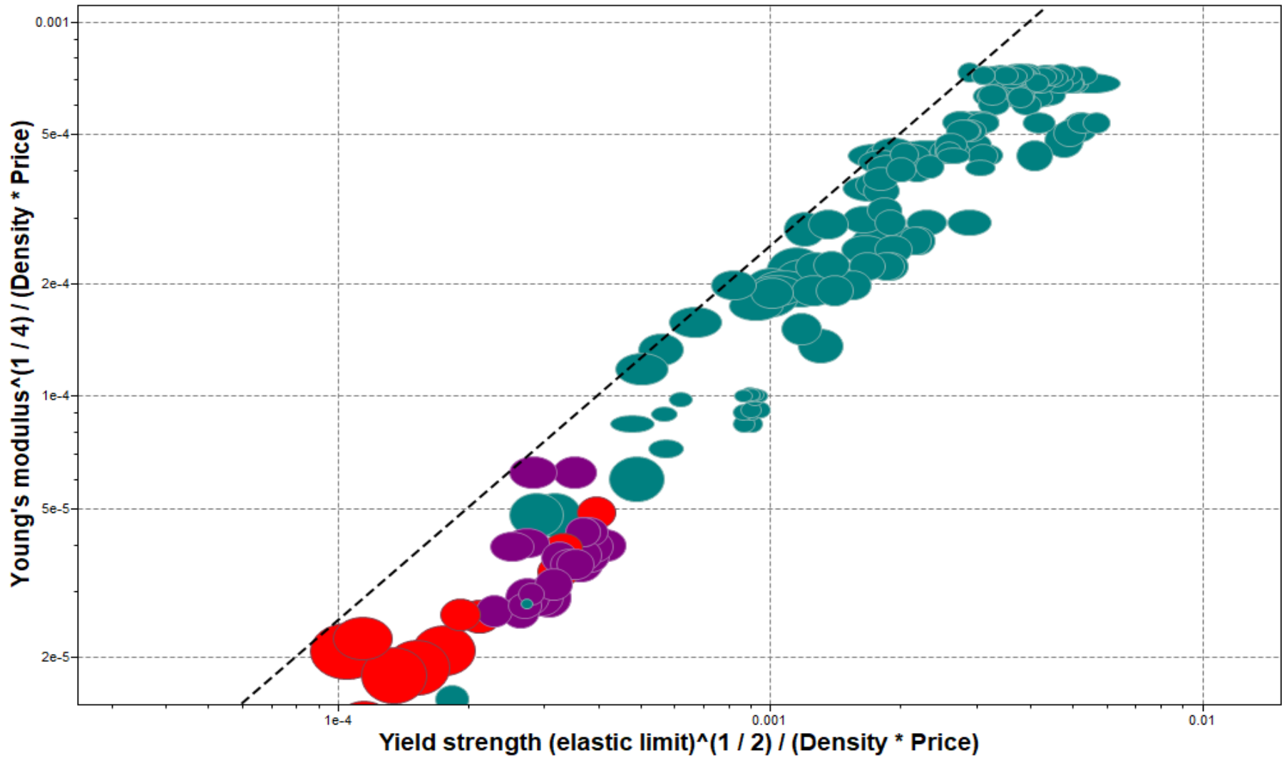
Figure (b) optimum selection using tangent line for pareto solution
