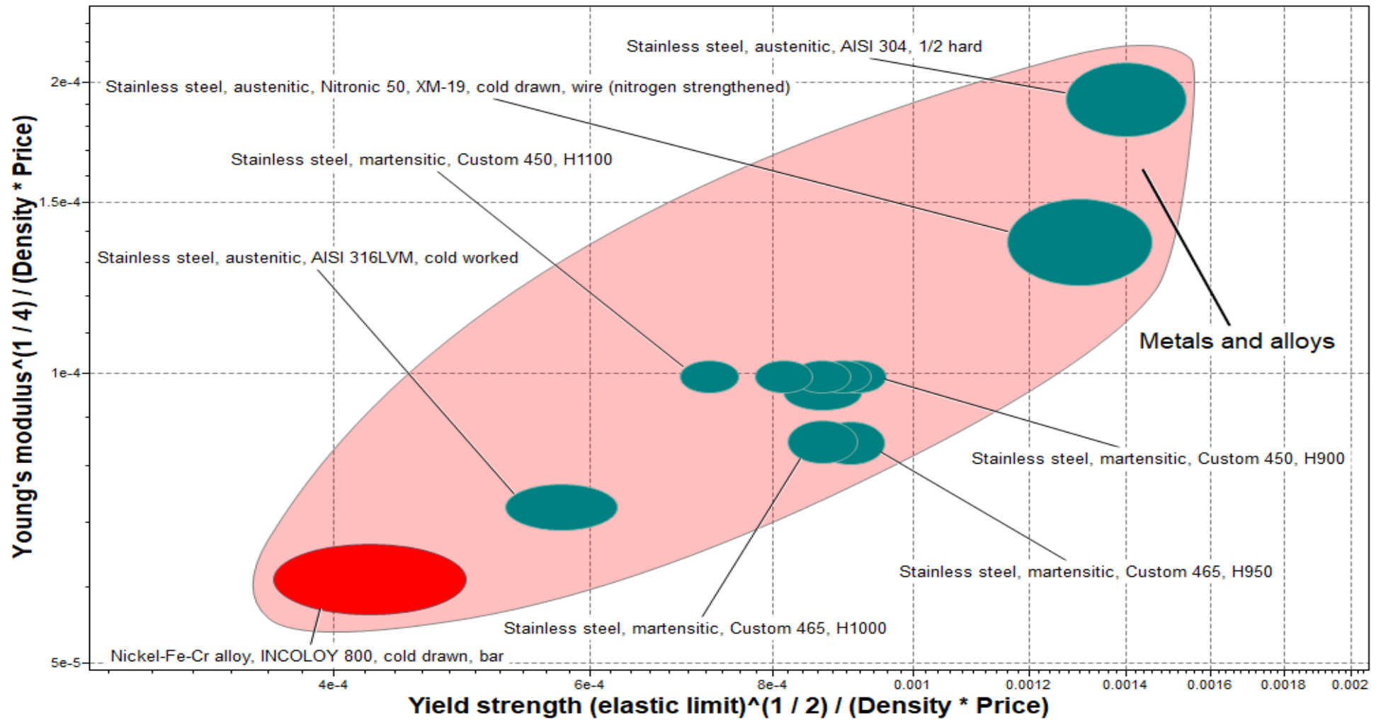
Figure (b) shortlisted materials for high sour oil and gas wells.
