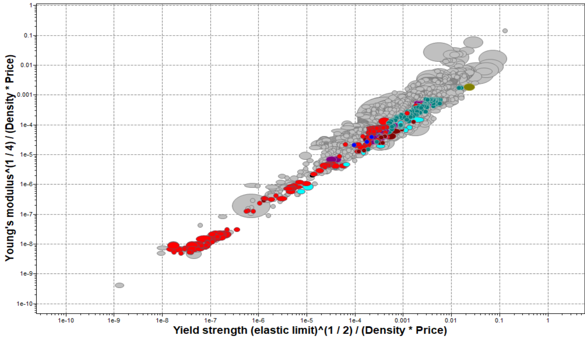
Figure 9 (a) The shortlisted materials for shale gas wells with high impact energy and temperature
