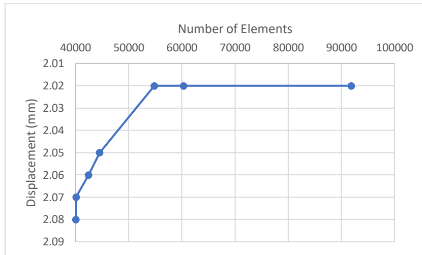
Figure 5 Mesh sensitivity study to ensure simulation result accuracy.
