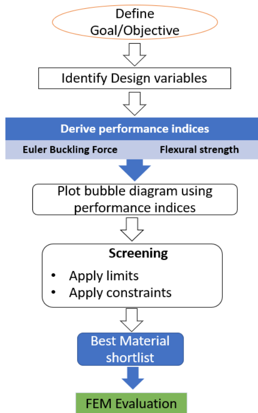
Figure 3: Casing material selection process for shale gas wells
