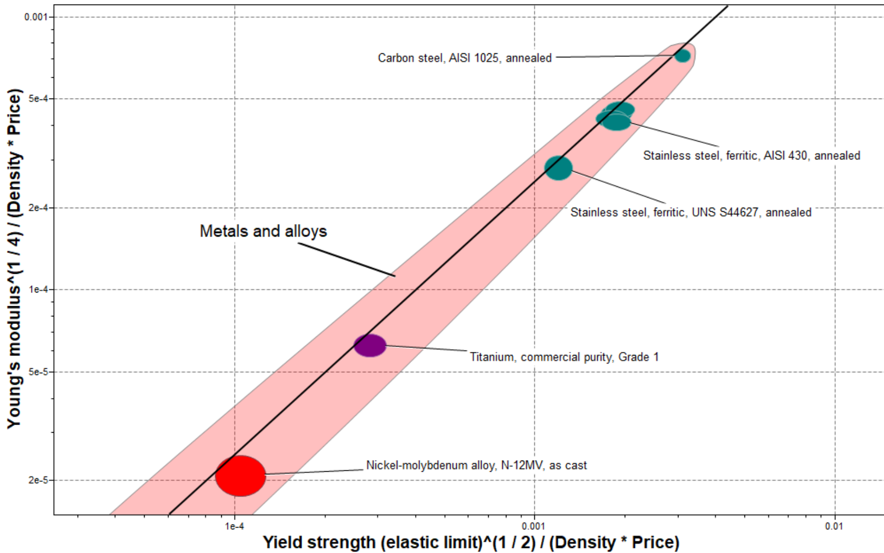
Figure 10 (b) the family envelope of the shortlisted material brittleness for high impact shales.
