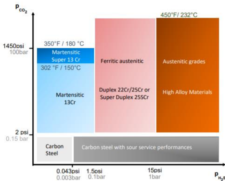
Figure 1 Simplified material selection chart (Millet et al. 2020).
