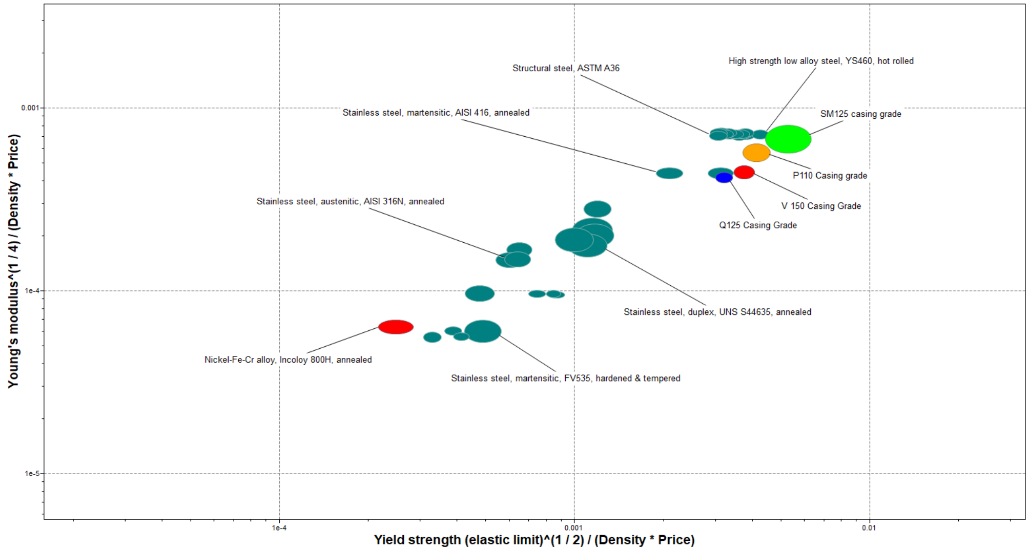
Figure 7 (a) the shortlisted candidates for shale gas well casing
