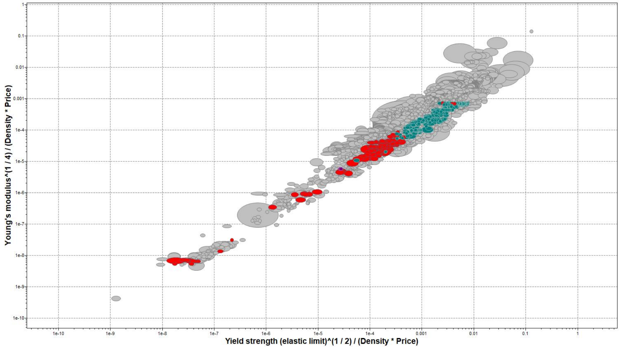
Figure 8 (a) The initial screening for the second scenario - induced stress and corrosion
