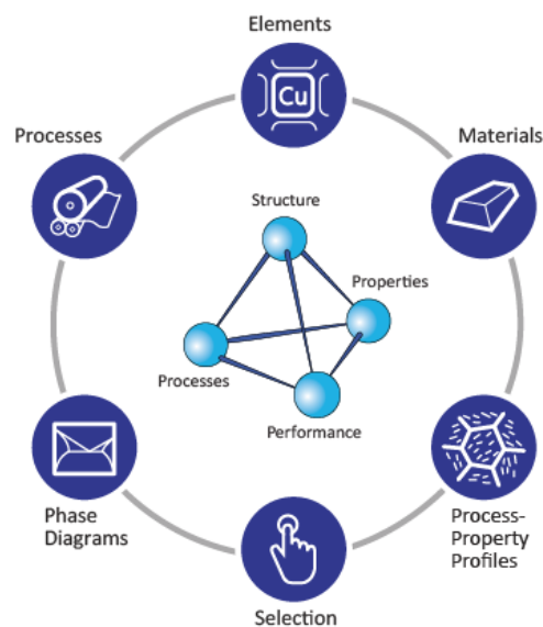
Figure 2 Data-structure of the CES for Material Science and Engineering database (Ashby, et al. 2018).
