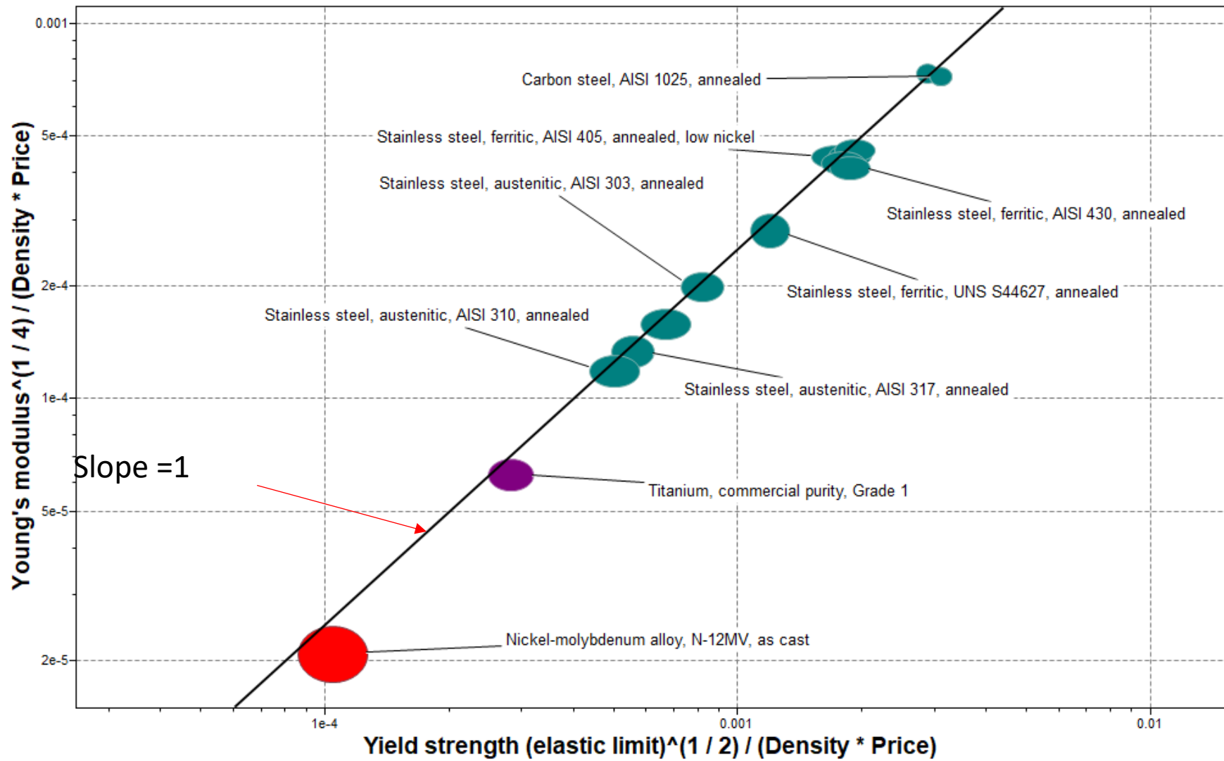
Figure 10(a) The shortlisted materials for shale gas wells with high impact potentials and service temperature
