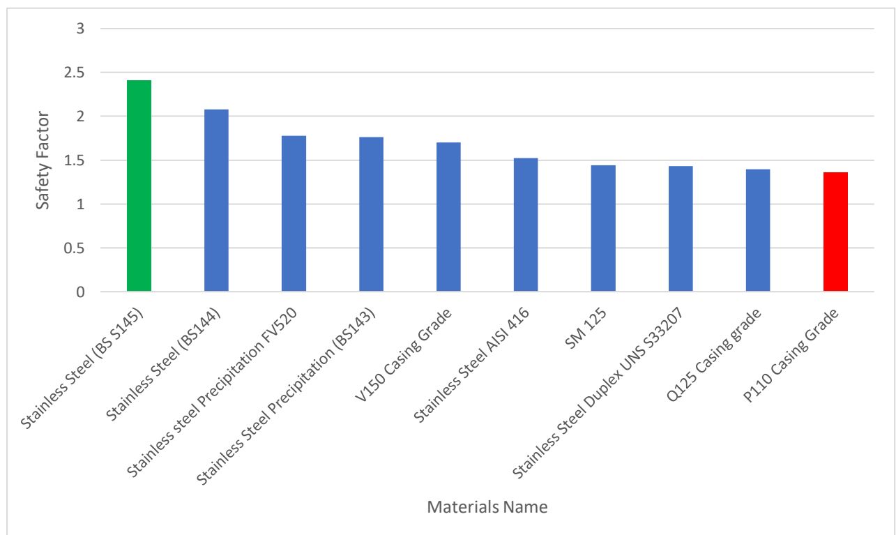
Figure 12 show safety factor for the 10 shortlisted materials as evaluated from FEM for each material.
