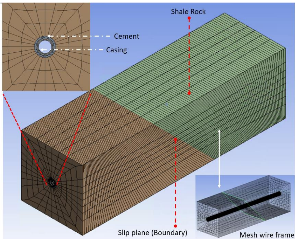
Figure 6 Finite element Model (54816 elements and 286352 nodes) showing casing, cement, rock and slip plane.
