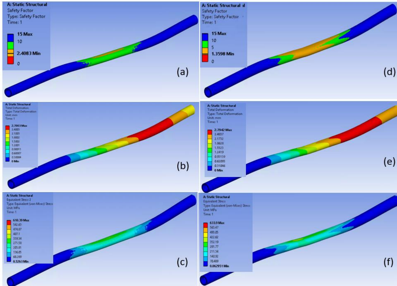
Figure 11 Comparison between Stainless steel (BS145) with P110 Casing grade showing (a) safety factor for -BS145 (b) Total Displacement-BS145 (c) von Mises stress - BS145 (d) safety factor -P110 (e) displacement -P110 (f) von Mises stress
