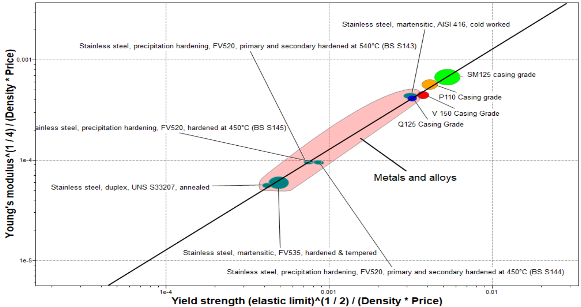
Figure 7(b) top ten (10) materials after further optimisation
