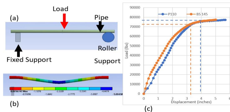
Figure 4: 3-point bending load displacement curve for P110 and BS 145 (a) Physical model (b) deform numerical model (c) Load versus displacement for P110 and BS145.
