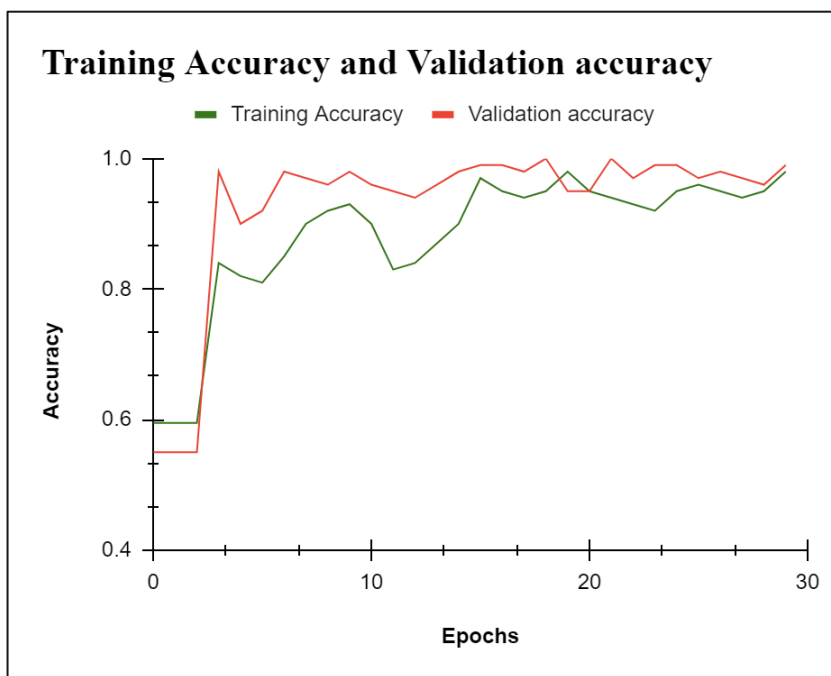
Fig. 9. Training and Validation Accuracy for 30 Epochs.
