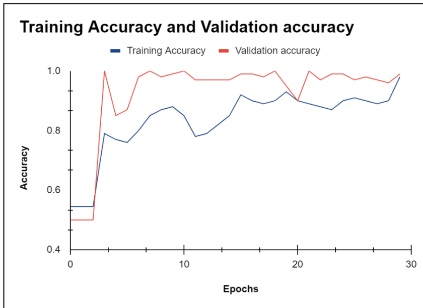
Fig. 12. Training and Validation Accuracy for 30 Epochs.
