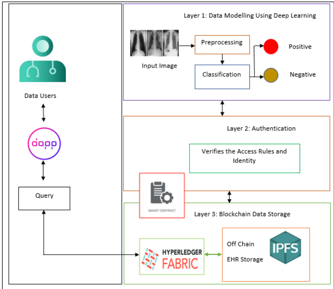
Fig. 1. Proposed Framework.
