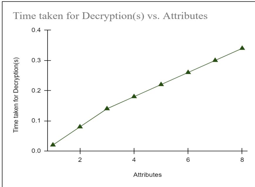
Fig. 7. Time taken for Decrypting Electronic Health Data.
