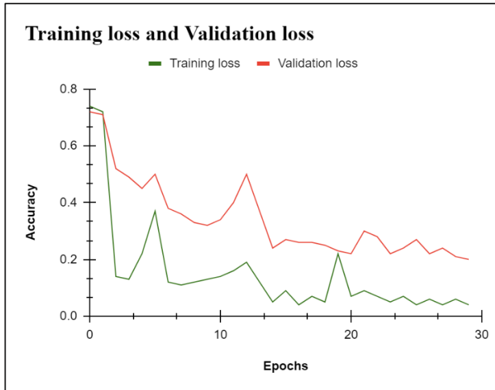
Fig. 10. Training and Validation loss for 30 Epochs.
