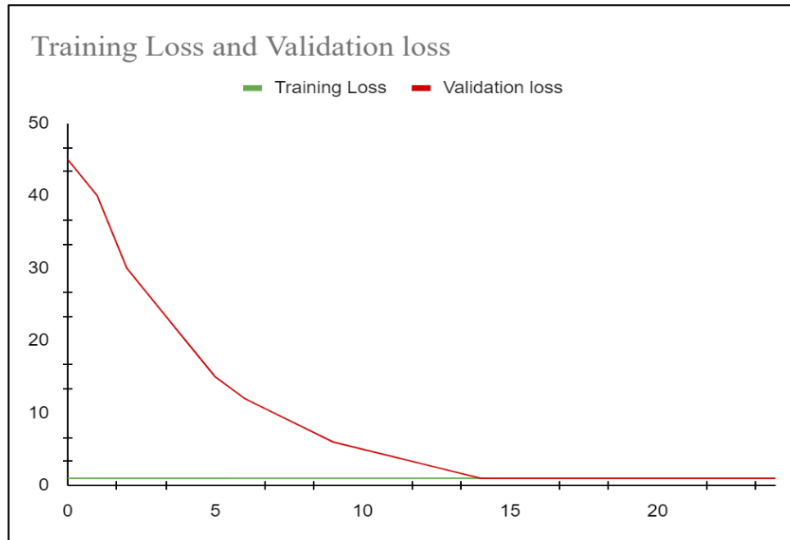
Fig. 16. Training and Validation loss for 25 Epochs.
