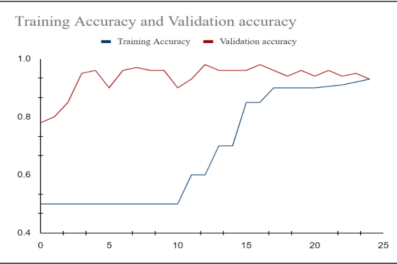
Fig. 15. Training and Validation Accuracy for 25 Epochs.
