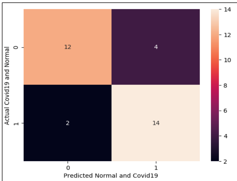
Fig. 8. Confusion matrix of prediction for Experiment 1.
