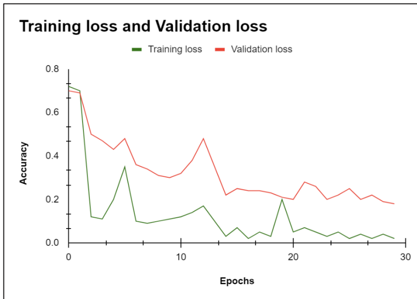
Fig. 13. Training and Validation loss for 30 Epochs.
