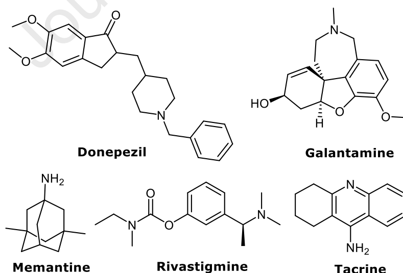
Figure 4 Chemical structures of the four current clinically available AD therapeutics (donepezil, galantamine, memantine, rivastigmine), and the first AChE inhibitor (tacrine) which was withdrawn in 2013 due to hepatotoxicity.
