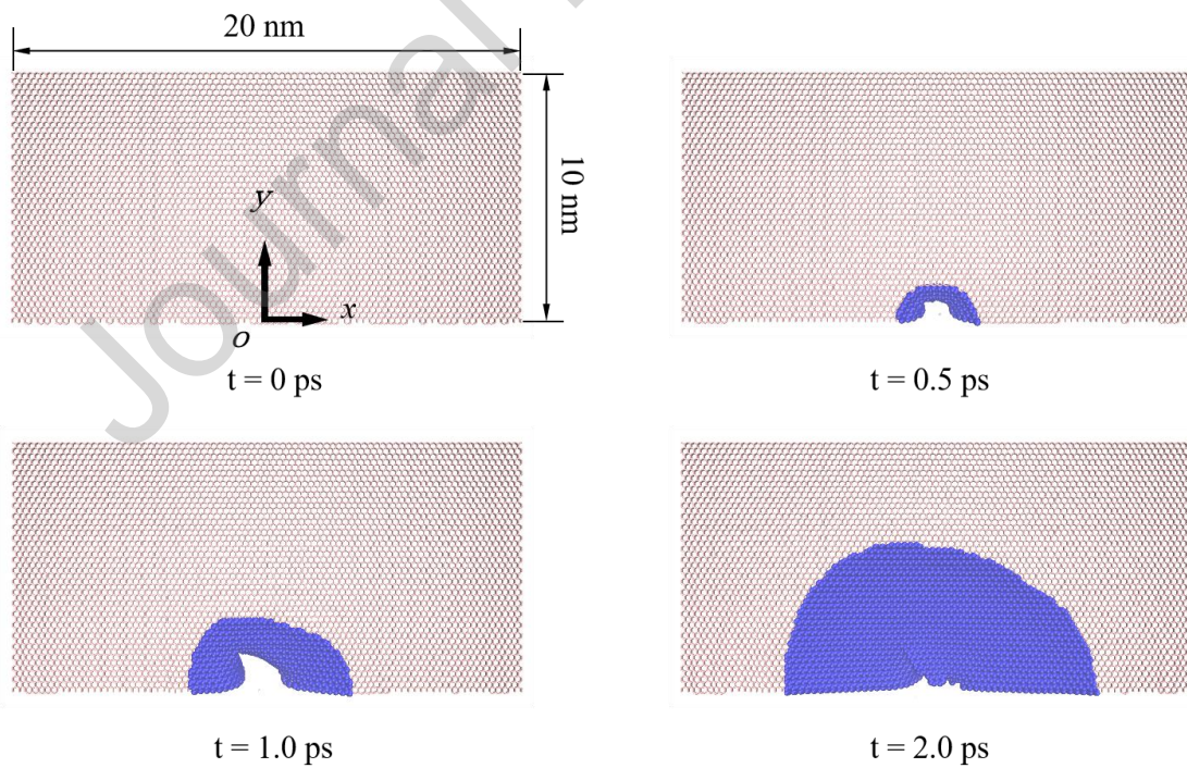
Fig. 13. Crack formation process of graphene impacted by projectile ( C_{180} ) with 5 km/s. (The blue regions represent the wave propagation area)
