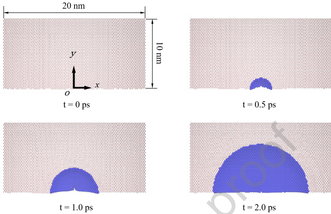
Fig. 12. Cone wave formation process of graphene impacted by projectile ( C_{180} ) with 4.5 km/s. (The blue regions represent the wave propagation area)
