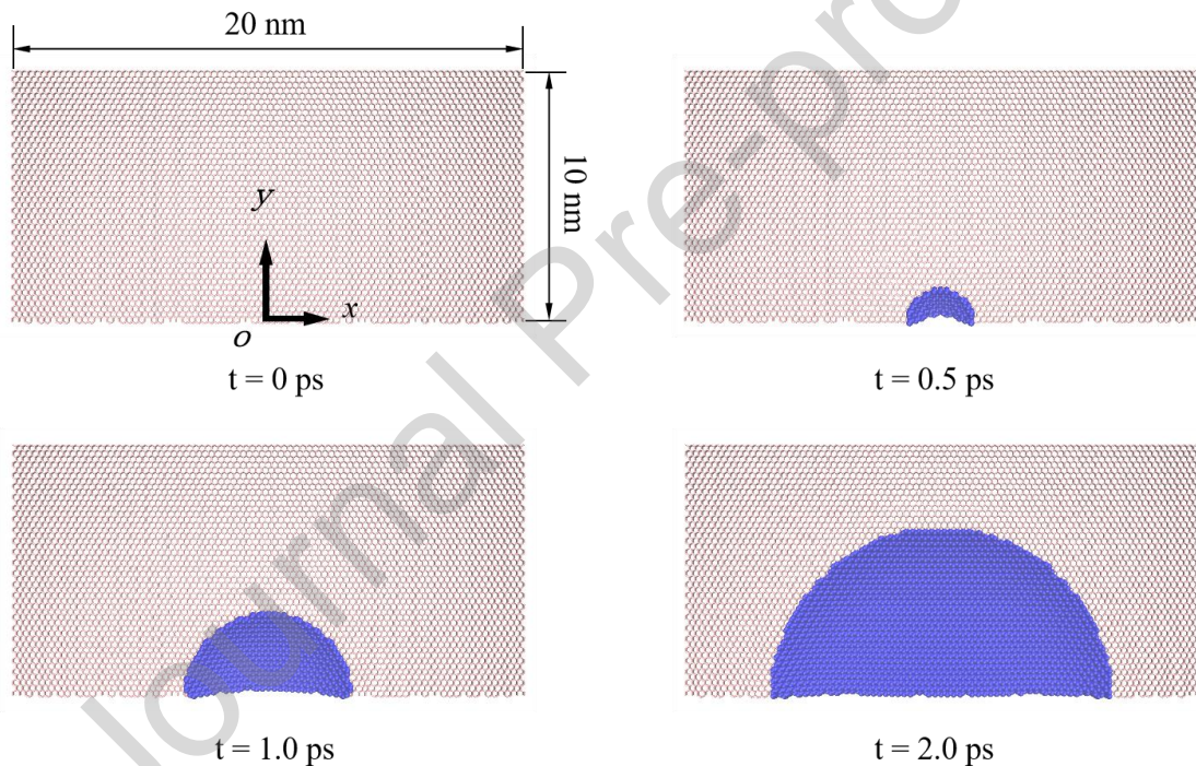
Fig. 11. Cone wave formation process of graphene impacted by projectile ( C_{180} ) with 4 km/s. (The blue regions represent the wave propagation area)
