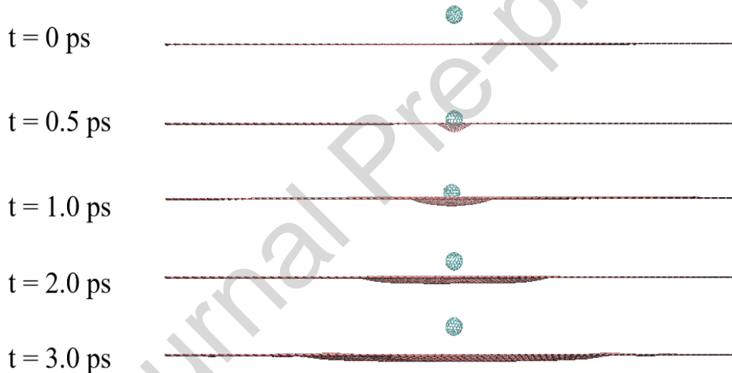
Fig. 7. Process of graphene impacted by projectile with 4 km/s.
