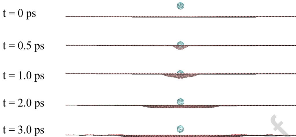
Fig. 8. Process of graphene impacted by projectile with 4.5 km/s.
