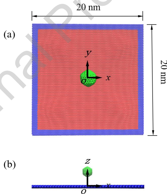
Fig. 1. Schematic of the impact simulation setup. The blue regions represent the fixed boundaries.
