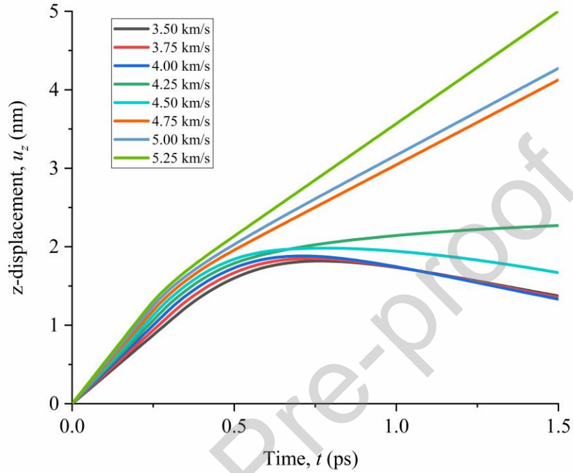
Fig. 4. Displacement-time history of fullerene projectile during impact
