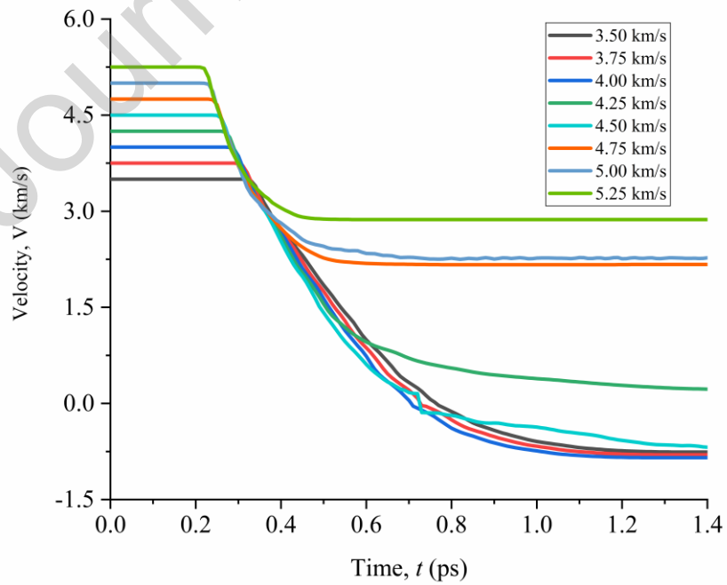
Fig. 5. Velocity-time history of fullerene projectile during impact
