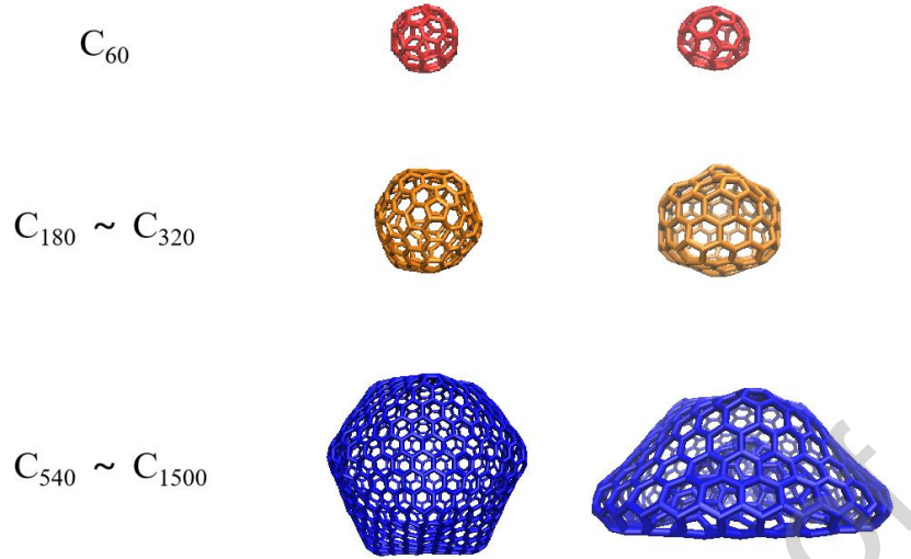
Fig. 3. Three types of buckling deformation of fullerene during impact. Left: the initial state of fullerenes before impact and Right: the state of fullerene at maximum deformation after impact
