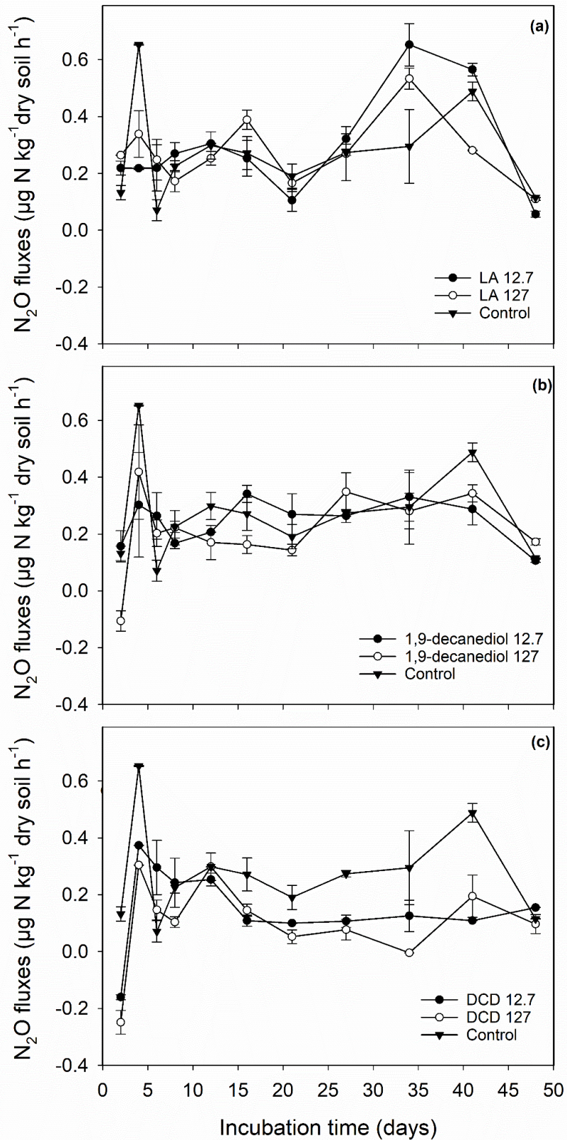
Fig. 3.2 Effect of different concentrations of LA (panel a), 1,9-decanediol (panel b) and DCD (panel c) on soil N 2 O emissions during a 48-d incubation at 10 °C. Error bars represent standard error of the mean (n=3).
