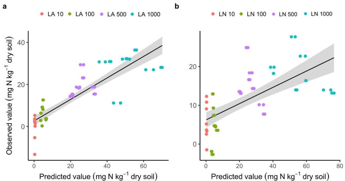
Fig. 4.5 Relationship between predicted and observed N immobilization in the linoleic acid (LA, panel a) and linolenic acid (LN, panel b) treatments. LA: y=0.51x+2.67 , R^2=0.74 ; LN: y=0.21x+6.24 , R^2=0.42 .
