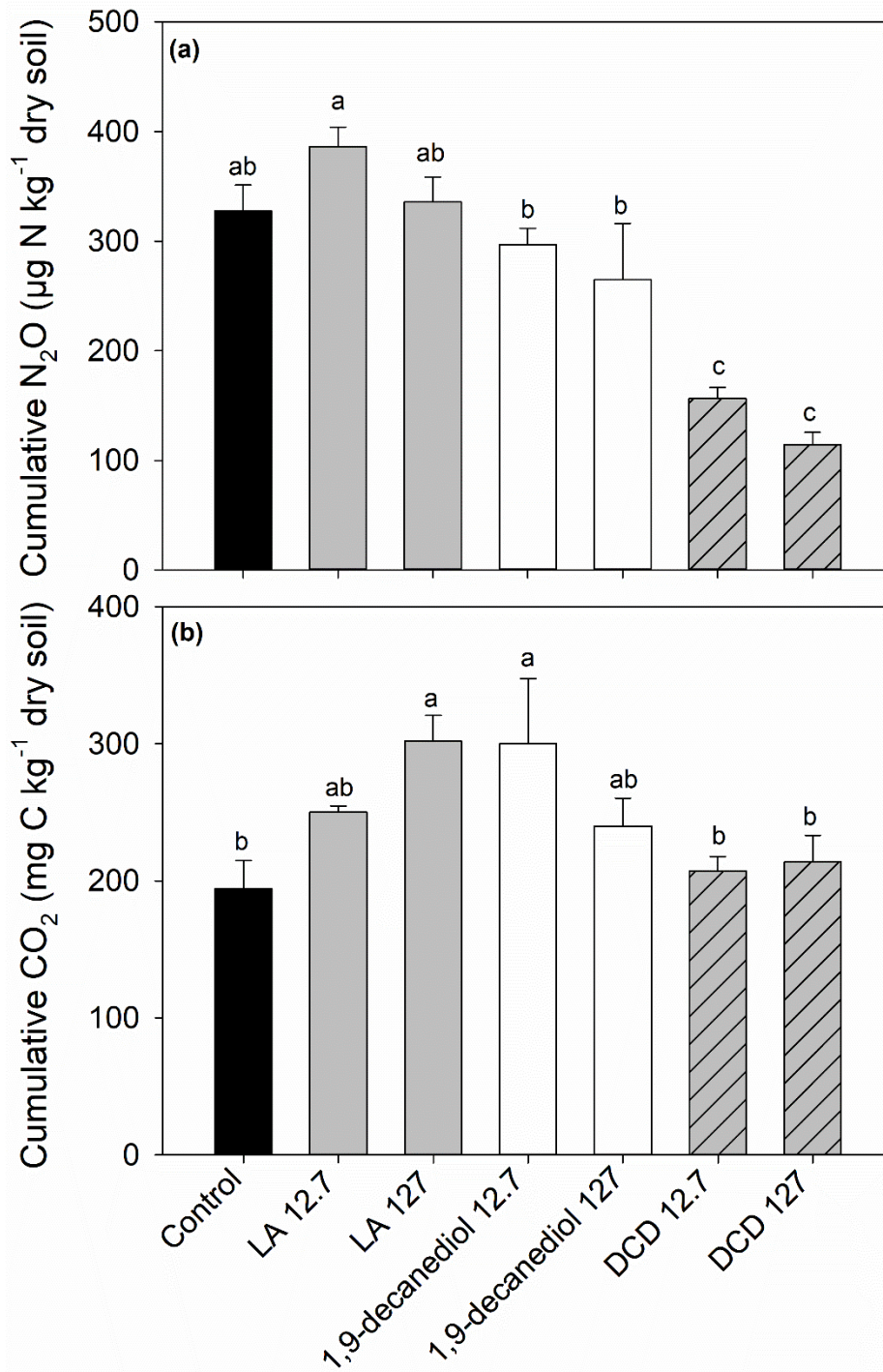
Fig. 3.3 Effect of LA, 1,9-decanediol and DCD on soil cumulative N 2 O (panel a) and CO 2 (panel b) emissions during a 48-d incubation at 10 °C. Error bars represent standard error of the mean (n=3).
