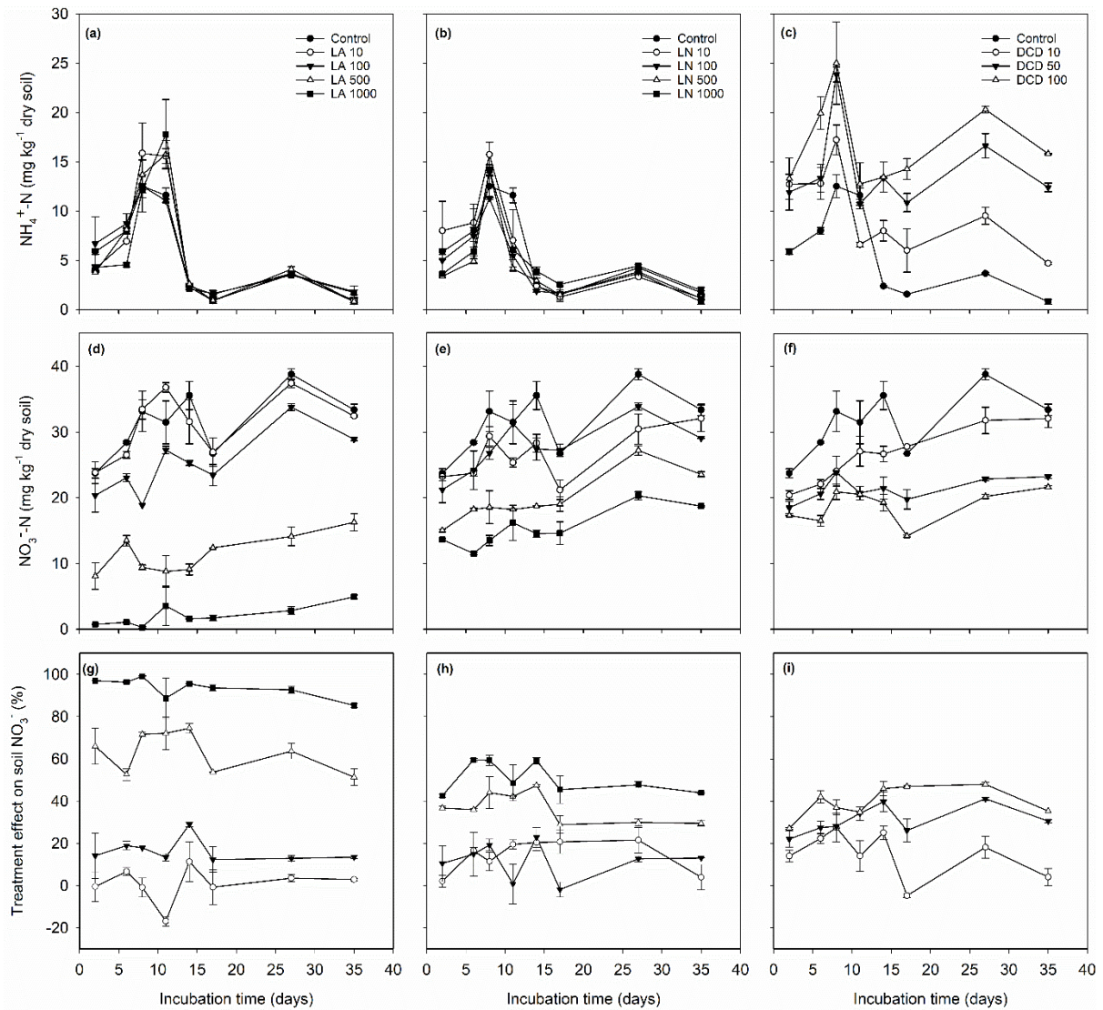
Fig. 4.1 Effect of different concentrations of linoleic acid (LA, panels a, d, g), linolenic acid (LN, panels b, e, h) and DCD (panels c, f, i) on soil \text{NH}_4^+ , \text{NO}_3^- concentrations and treatment effect on soil \text{NO}_3^- concentration during a 38-d incubation at 10 °C. Error bars represent standard error of the mean (n=4).
