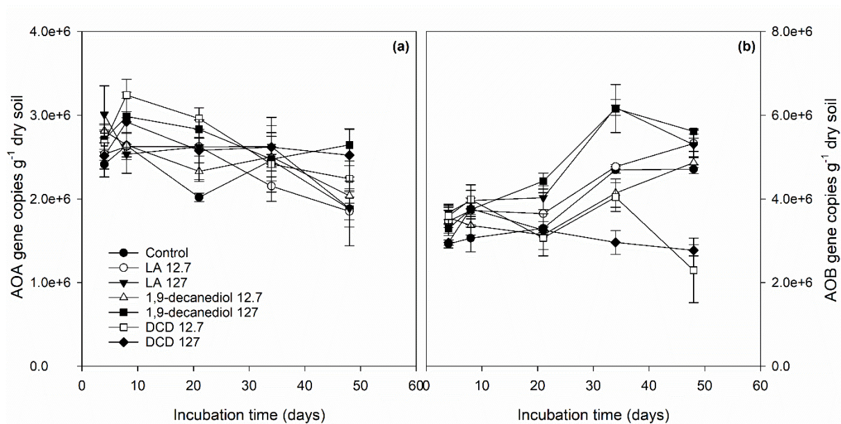
Fig. 3.5 Effect of LA, 1,9-decanediol and DCD on gene copies of AOA (panel a), AOB (panel b) during a 48-d incubation at 10^\circ\text{C} . Error bars represent standard error of the mean ( n=3 ).
