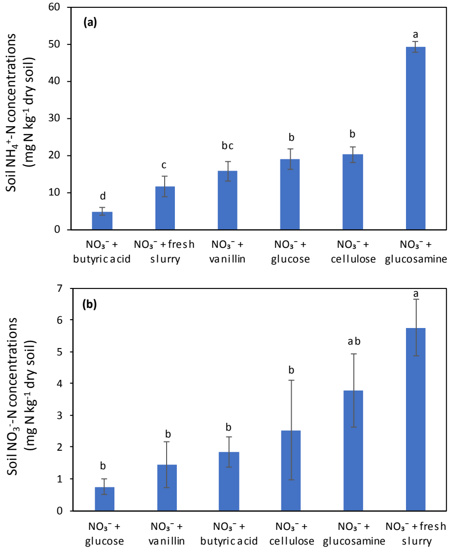
Fig. 6.3 Soil NH 4 + (panel a) and NO 3 - (panel b) concentrations in the NO 3 - + glucose (positive control) and NO 3 - + C sources (vanillin, cellulose, glucosamine, butyric acid and fresh slurry) treatments at the end of the incubations. Error bars represent the standard error of the mean (n=4). Different letters indicate the significant differences between the treatments at P < 0.05 by LSD. Note different y-axis units between the NH 4 + -N and NO 3 - -N panels.
