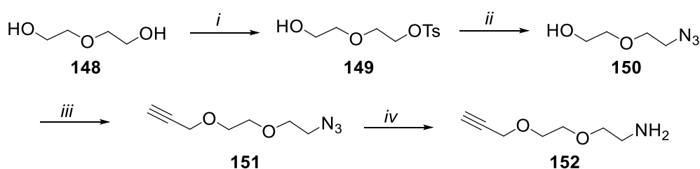
Scheme 42: A synthetic route from DEG to produce the bifunctional linker 152 in a yield of 34 % over 4 steps. i. TsCl, Et 3 N, DCM, 78%; ii. NaN 3 , DMF, 90%; iii. propargyl bromide, NaH, DMF, 78%; iv. PPh 3 , H 2 O, 63%.
