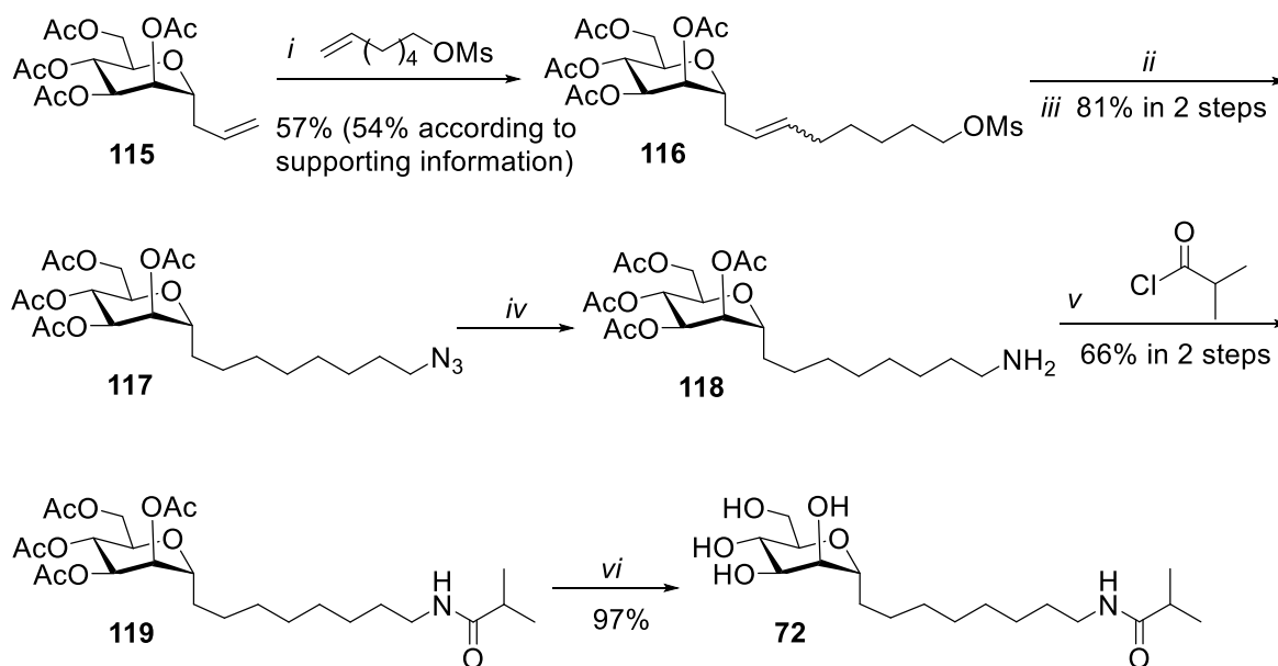
Scheme 26: Synthesis of the \alpha - C -mannopyranoside. i. Grubbs 2nd, 10%, DCM, reflux, 8 h; ii. H 2 , Pd/C, MeOH, 4 h; iii. NaN 3 , DMF, 80°C, overnight; iv. H 2 , Pd/C, MeOH, 10 h; v. isobutyric chloride, pyridine, DMAP, 5.h; vi. NaOMe, MeOH, 4 h, Amberlite IR120 (H). 65
