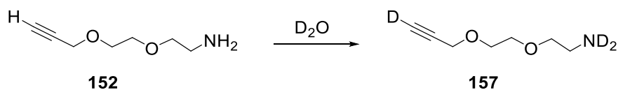
Scheme 44: Possible deuterium-proton exchange of the alkyne proton of 152 in \text{D}_2\text{O} .
