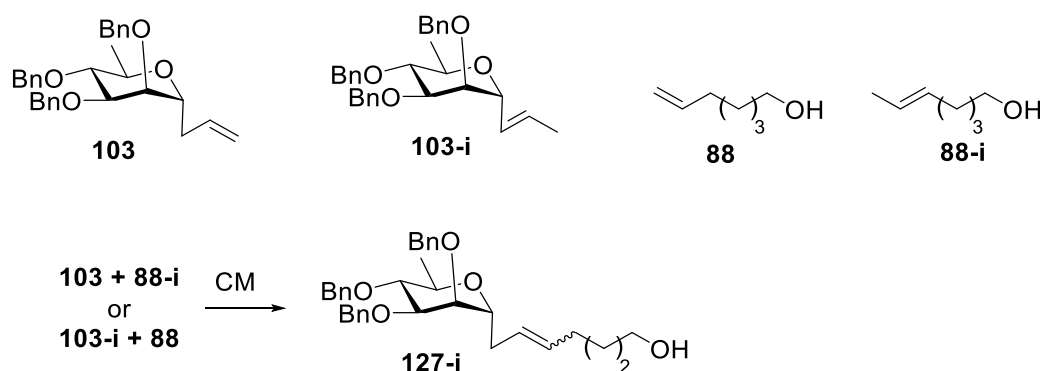
Scheme 33-i: Possible isomers of the olefins 103 and 88 and the CM product 127-i results in the loss of one carbon in the linker.
