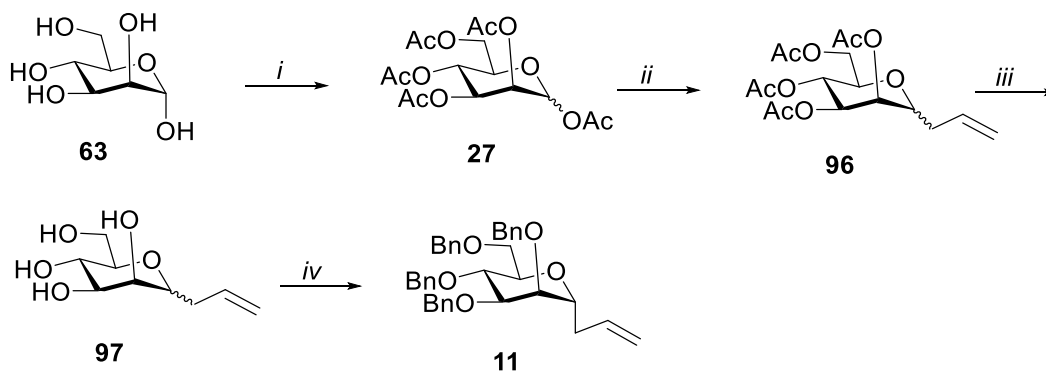
Scheme 21: i. Ac 2 O, pyridine, DMAP (rt, 2h), 97%; ii. allyltrimethylsilane, BF 3 ·Et 2 O, TMSOTf, CH 3 CN, 95%; iii. NaOMe, MeOH (rt), 91%; iv. BnBr, NaH, DMF, 81%.
