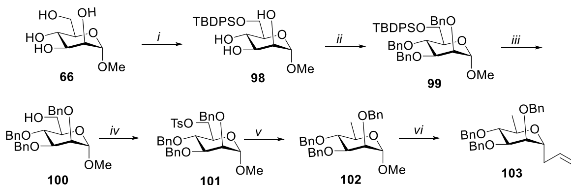
Scheme 22: i. TBDPSCl, imidazole, DMF, (rt, overnight), 83%; ii. BnBr, NaH, DMF, 50%; iii. TBAF, THF, 75%; iv. TsCl, DMAP, pyridine, DCM, 85%; v. LAH, ether, 62%; vi. allyltrimethylsilane, TMSOTf, CH 3 CN, 86%.
