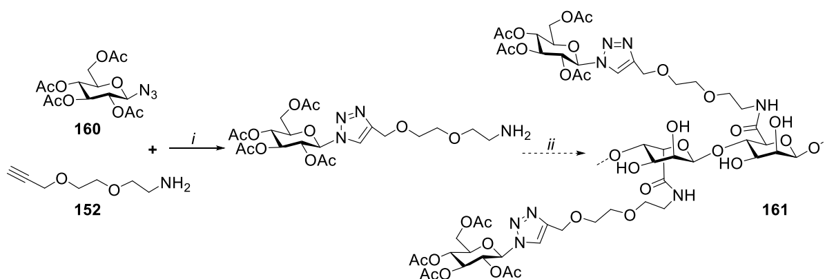
Scheme 46: A model sugar 160 to confirm that the click reaction was working. i . \text{CuSO}_4 , NaAsc, THF/ \text{H}_2\text{O} (1:1), stirring, rt., 1h; ii . EDC, NHS, \text{H}_2\text{O} (stirring, rt, overnight).
