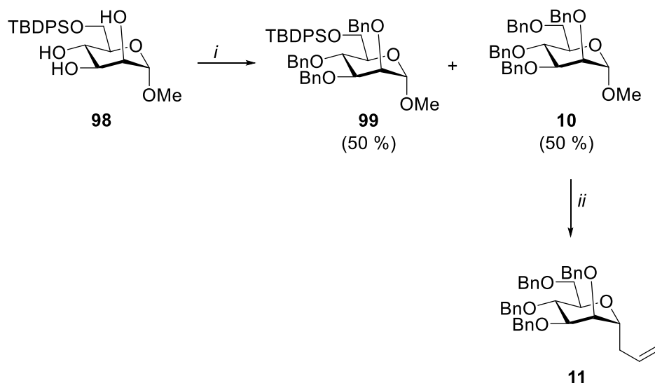
Scheme 23: i. BnBr, NaH, DMF, 50% and side product 10 50%; ii. allyltrimethylsilane, TMSOTf, CH 3 CN, 70%.
