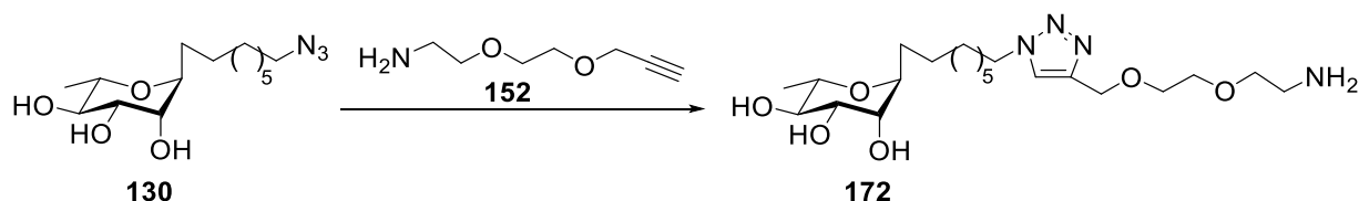
Scheme 56: The click reaction of the compound 130 with the linker 152 using \text{CuSO}_4 and sodium ascorbate.
