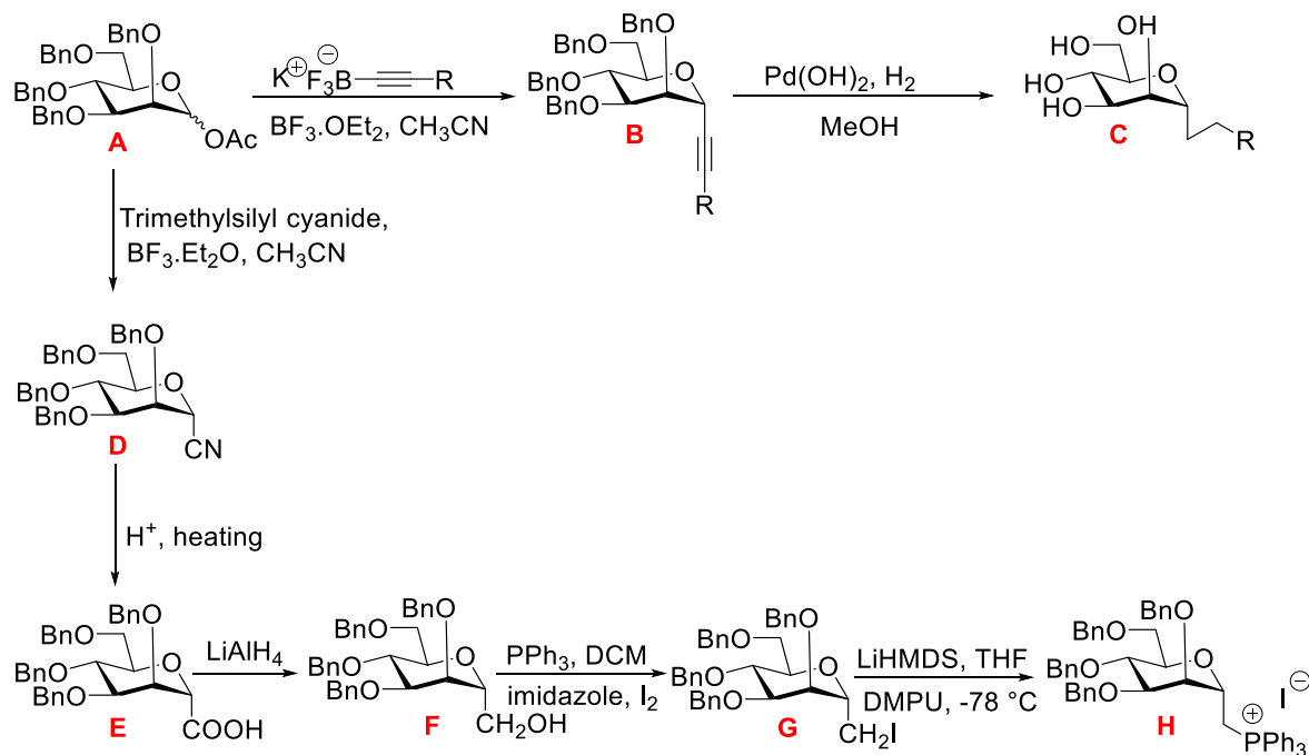
Scheme 5.A: Suggested synthetic route to Wittig salt OR coupling a Wittig salt H as coupling partner with a linker of aldehyde I (see Scheme 5.B ).
