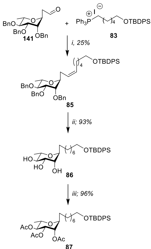
Scheme 17: i. LiHMDS, THF, DMPU, -78 °C; ii. Pd(OH) 2 /C, EtOAc/ MeOH(1:1); iii. Ac 2 O, pyridine.
