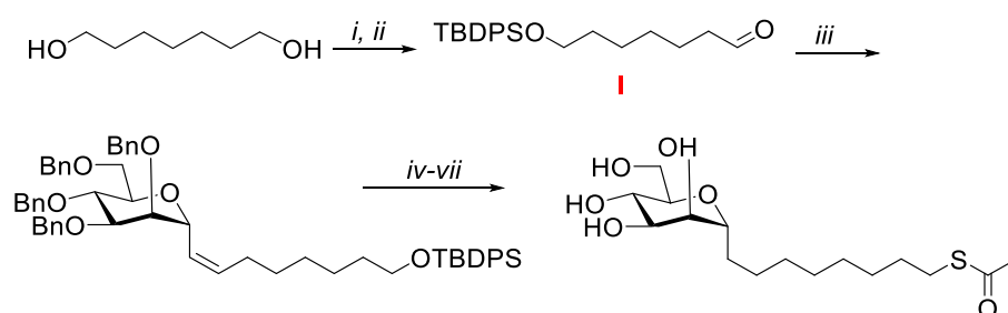
Scheme 5.B: Suggested synthetic route for Wittig coupling and a direct introduction of a thio acetate group. i. TBDPSCl , DIPEA , DMF , overnight, rt ; ii. Cr_2O_3 , H_2SO_4 , H_2O ; iii. H , LiHMDS , THF , DMPU , -78^\circ C ; iv. TBAF , THF , rt ; v. TsCl , pyridine , rt ; vi. potassium thioacetate, DMF , rt ; vii. Pd(OH)_2/C , EtOAc/MeOH(1:1) , rt .
