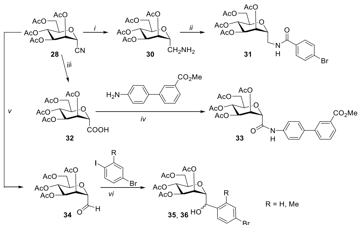
Scheme 8: Synthesis of C-mannosides from cyanomannoside: i. LiAlH 4 , THF, rt; ii. 4-bromobenzoyl chloride, pyridine, rt; iii. 25% HCl aq, 50 °C; iv. HATU, DIPEA, 0 °C to rt, DMF; v. DIBAL, DCM, -78 °C; vi. BuLi Et 2 O, -78 °C to -20 °C.
