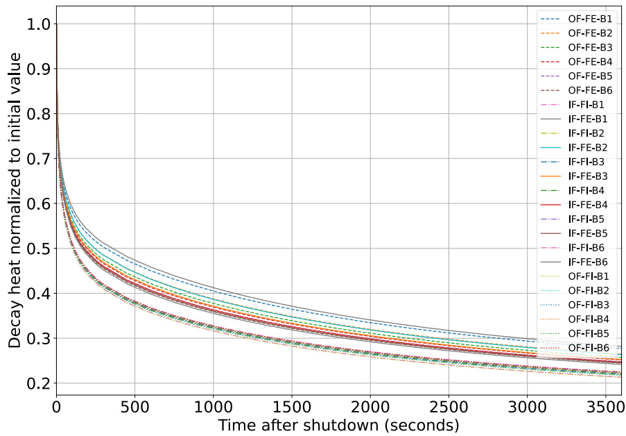
Fig. 8 Zone-wise decay heat evolution normalized to the initial value at the short-term.
