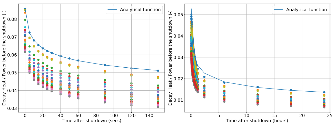
Fig. 17 Ratio between the decay heat and power prior to shutdown for fertile regions along with the derived analytical functions for cooling times up to 150 seconds (left) and from 150 seconds to 1 day (right).
