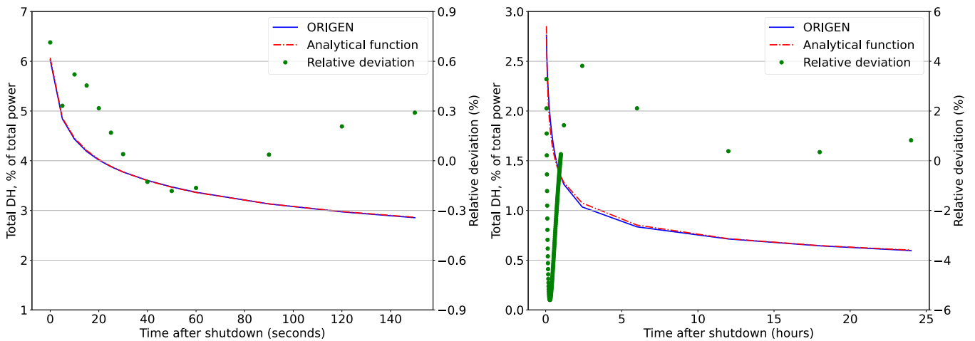
Fig. 19 Total decay heat calculated by ORIGEN compared to the total decay heat estimated by the analytical function for cooling times up to 150 seconds (left) and from 150 seconds to 1 day (right).
