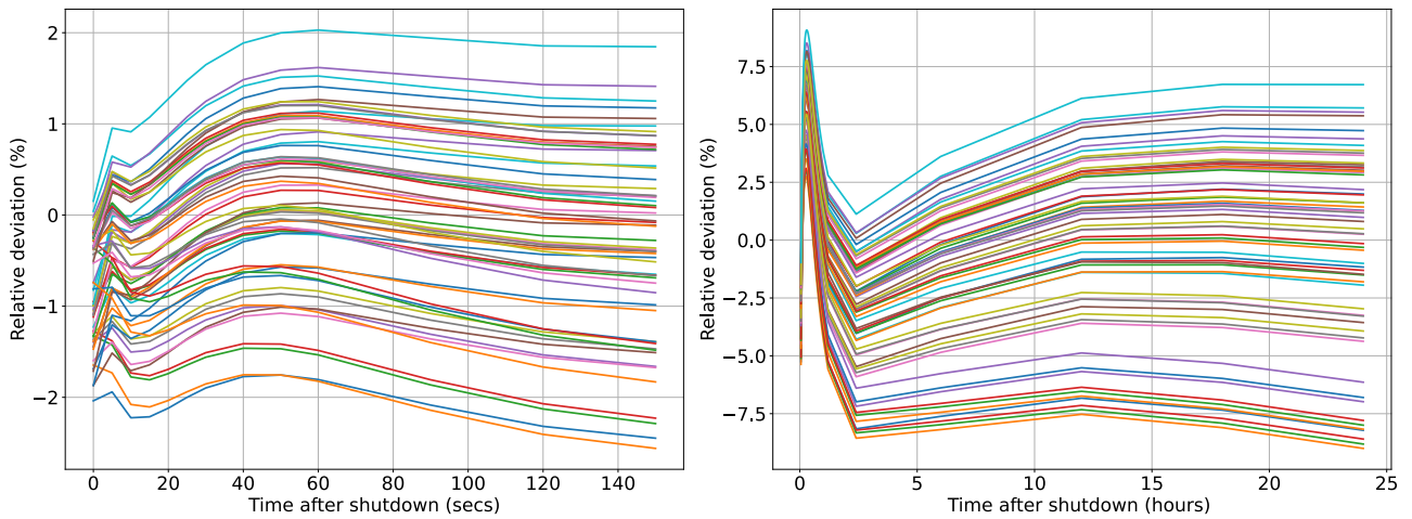
Fig. 16 Fissile regions: relative deviation between actual and estimated function-based decay heat for cooling times up to 150 seconds (left) and from 150 seconds to 1 day (right).
