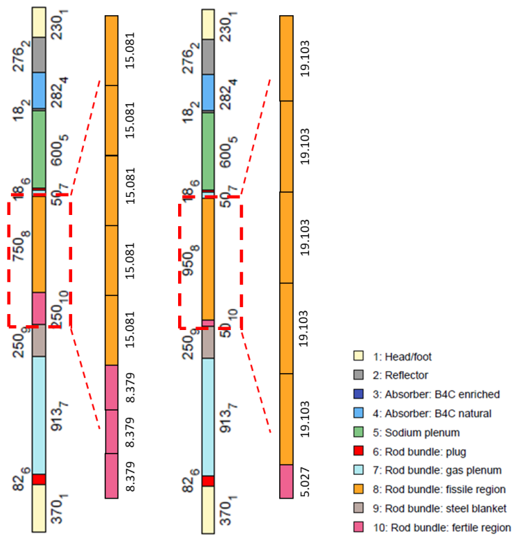
Fig. 2 Axial layout of IF (left) and OF (right) assemblies.
