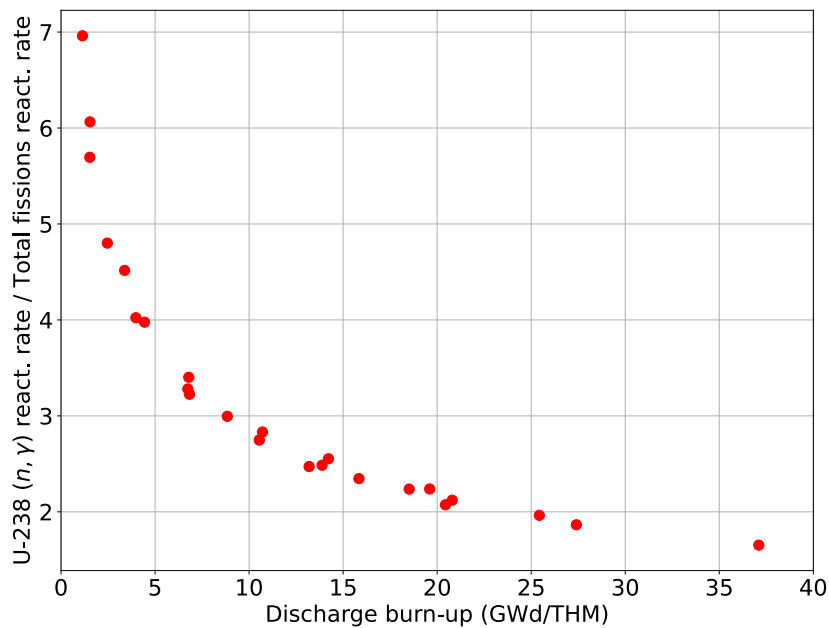
Fig. 14 Ratio of the U-238 capture rate to total fission rate as a function of discharge burnup for fertile zones.
