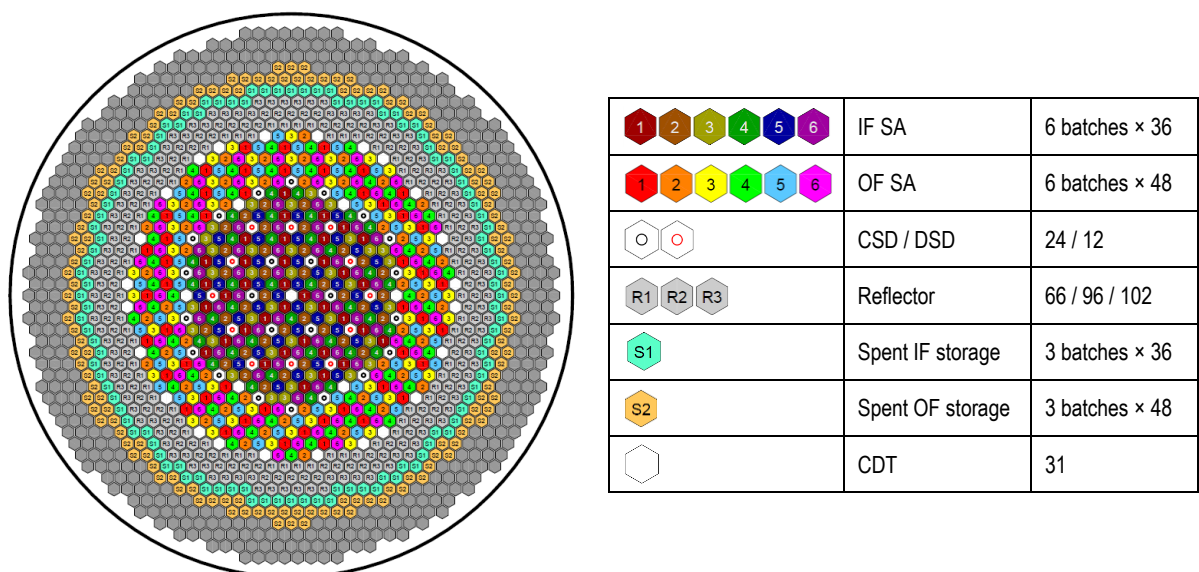
Fig. 1 Radial core layout
