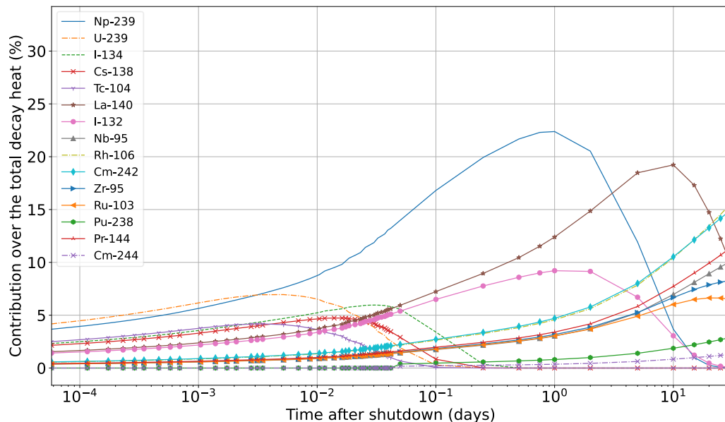
Fig. 10 Major nuclide contributors to the decay heat.
