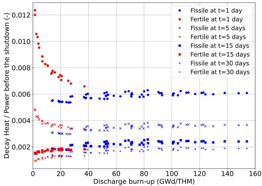
Fig. 13 Ratio between decay heat and power before the shutdown as a function of the discharge burnup for the 84 burnable materials at various cooling times within the mid-term.
