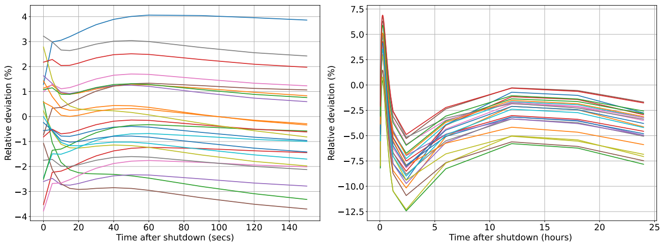
Fig. 18 Fertile regions: relative deviation between actual and estimated function-based decay heat for cooling times up to 150 seconds (left) and from 150 seconds to 1 day (right).
