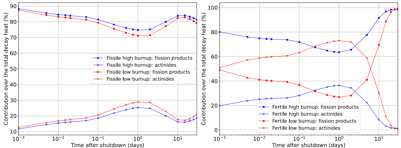
Fig. 12 Fission products and actinides contribution over the total decay heat for fissile (left) and fertile (right) materials at low and high burnup.
