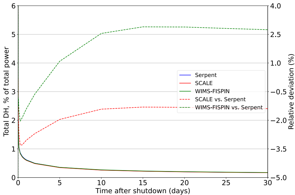
Fig. 4 Total decay heat normalized to nominal power in the mid-term.
