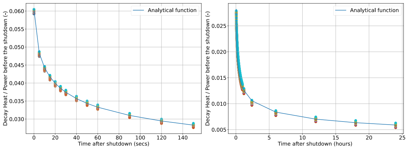
Fig. 15 Ratio between the decay heat and power prior to shutdown for fissile regions along with the derived analytical functions for cooling times up to 150 seconds (left) and from 150 seconds to 1 day (right).
