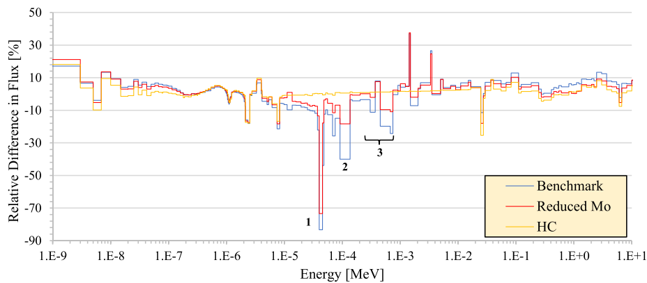
Fig. 4. Difference in normalized neutron flux in CR of UCam WIMS relative to GT Serpent.
