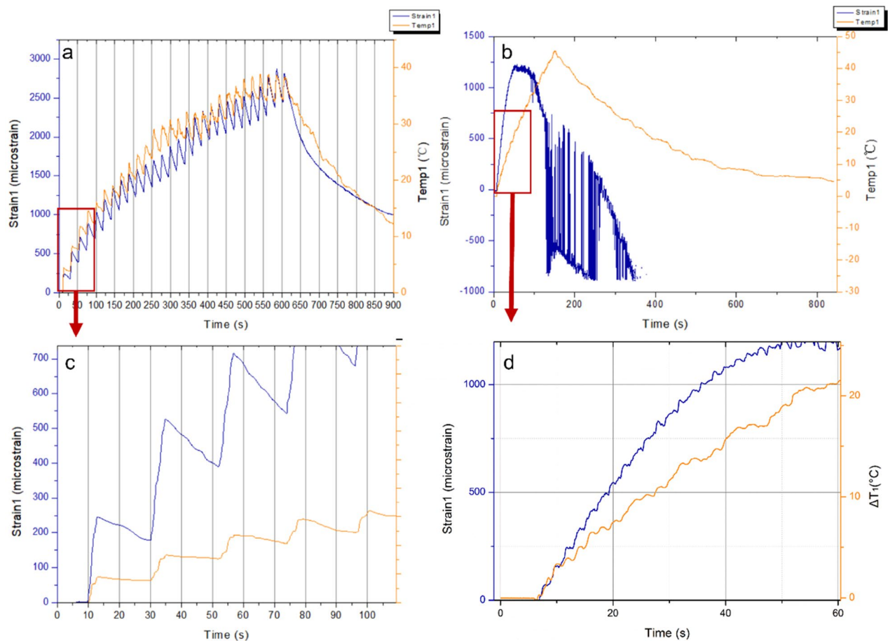
Figure 23. Strain and temperature measurements of FBG sensor 1 of (a) and (c) 15 wt.% BaTiO 3 /Epoxy nanocomposite sample under 100 W for 600 s, (b) and (d) 15 wt.% BaTiO 3 -Epoxy nanocomposite sample under 440 W for 148 s.
