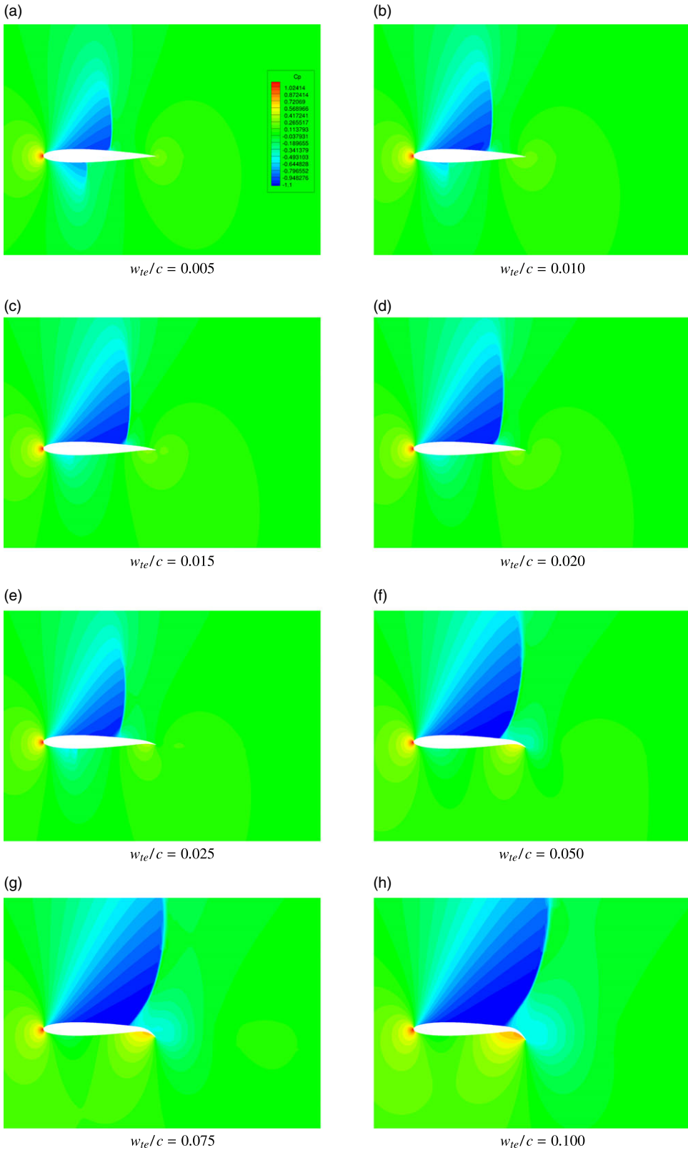
Figure 7. Pressure fields for different deflections at x = 0.8 , \alpha = 0^\circ , Re = 3 \times 10^6 and Ma = 0.8 .
