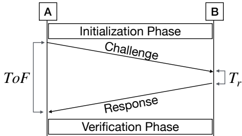
Fig. 6. Device A and B run a distance bounding protocol to acquire the time-of-flight (ToF) and measure the distance.
