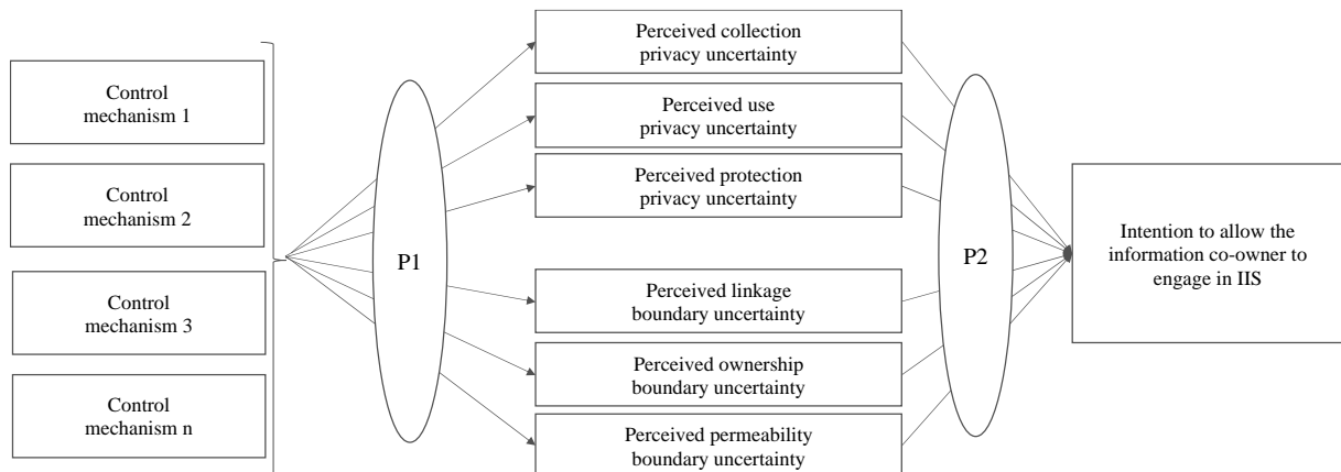
Figure 2. Research model.
