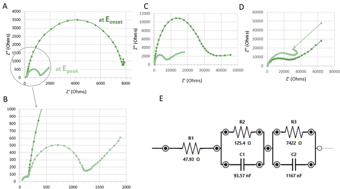
Fig. 10 Nyquist plot of 1 mM catalyst in electrolyte for \text{Co(II)Cl}_2 reference (A) and (B); [\text{Co}_6\text{Na}(\text{NCMe})_6(\mu\text{-O})(p\text{-tert-butylcalix[6]areneH})_2\text{Br}] \cdot 7\text{MeCN} (6·7MeCN) (C); [\text{Co}_4\text{Na}(\text{NCMe})_4(\mu\text{-O})(p\text{-tert-butylcalix[8]arene})(p\text{-tert-butylcalix[8]areneH}_5)\text{Br}] \cdot 13\text{MeCN} (7·13MeCN) (D) recorded in the presence of acetic acid substrate (orange; 2 mM equivalent with respect to catalyst concentration). The AC impedance was recorded at constant polarization of E_{\text{onset}} (dark green) and E_{\text{peak}} (pale green) as listed in Table 1 for corresponding catalyst. The electrical equivalent circuit used for fitting the impedance is displayed in (E). An example of fitting results to the proposed equivalent circuit with reported error of fitting is included in the ESI (Fig. S16†).
