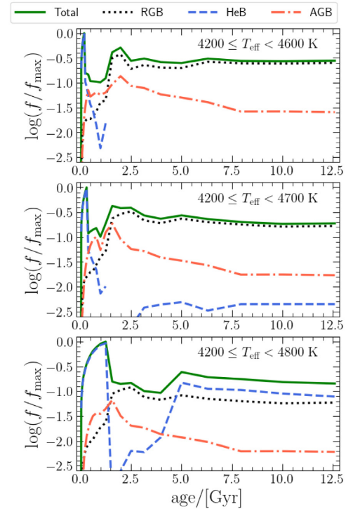
Figure 2. The selection factor f as derived from the PARSEC stellar evolutionary tracks (release v1.2S) with metallicity Z = 0.01 (Bressan et al. 2012; Tang et al. 2014; Chen et al. 2015), by assuming the IMF of Kroupa (2001). Different panels correspond to different maximum values of T_{\text{eff}} , from 4600 to 4800 K.
