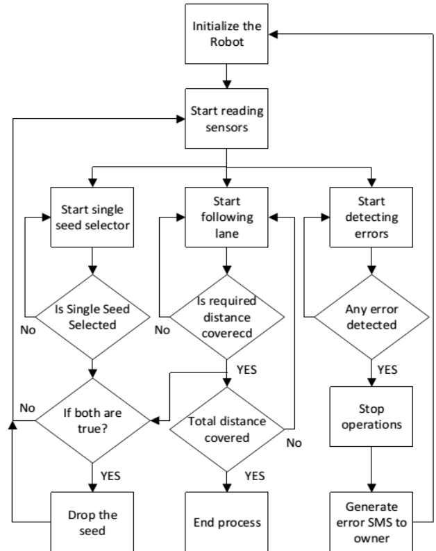
Fig. 8. Flow chart of the proposed software architecture
