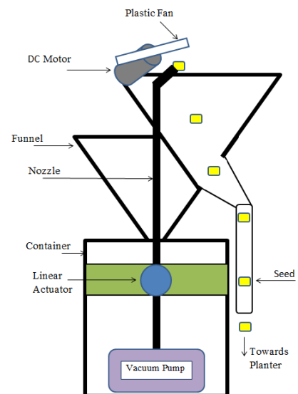
Fig. 5. Schematics of the proposed design of single seed selector
