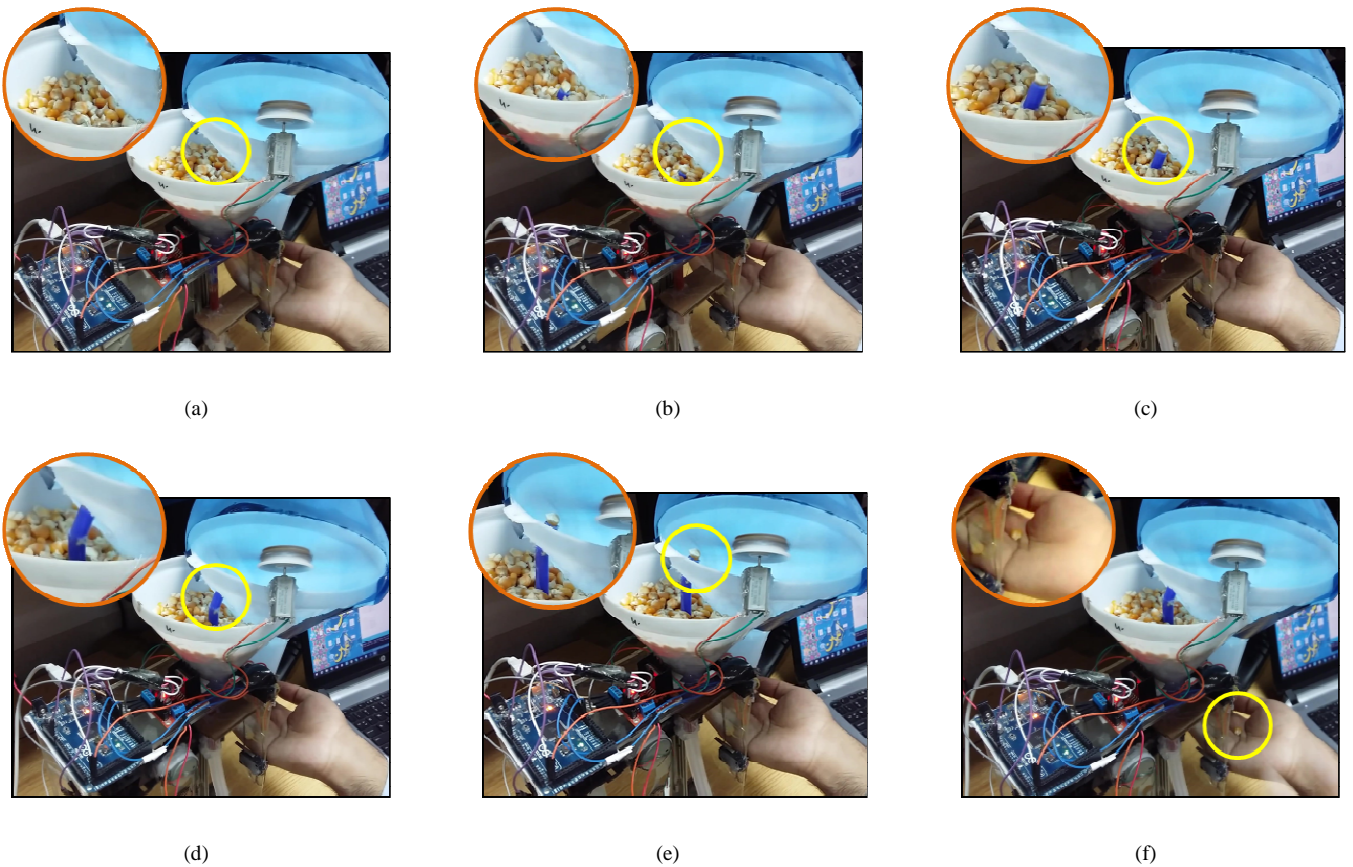
Fig. 10. Operation of single selector picking the single seed from the bulk. (a) Selector starts its process. (b) Selector starts to separate the single seed (c) Selector separated the single seed and nozzle goes upward to through it in to the other funnel. (d) Nozzle is about to enter the next funnel. (e) Nozzle takes the selected seed to the next funnel in order to through it down using the plastic fan. (f) Single seed is successfully reaches down through the funnel
