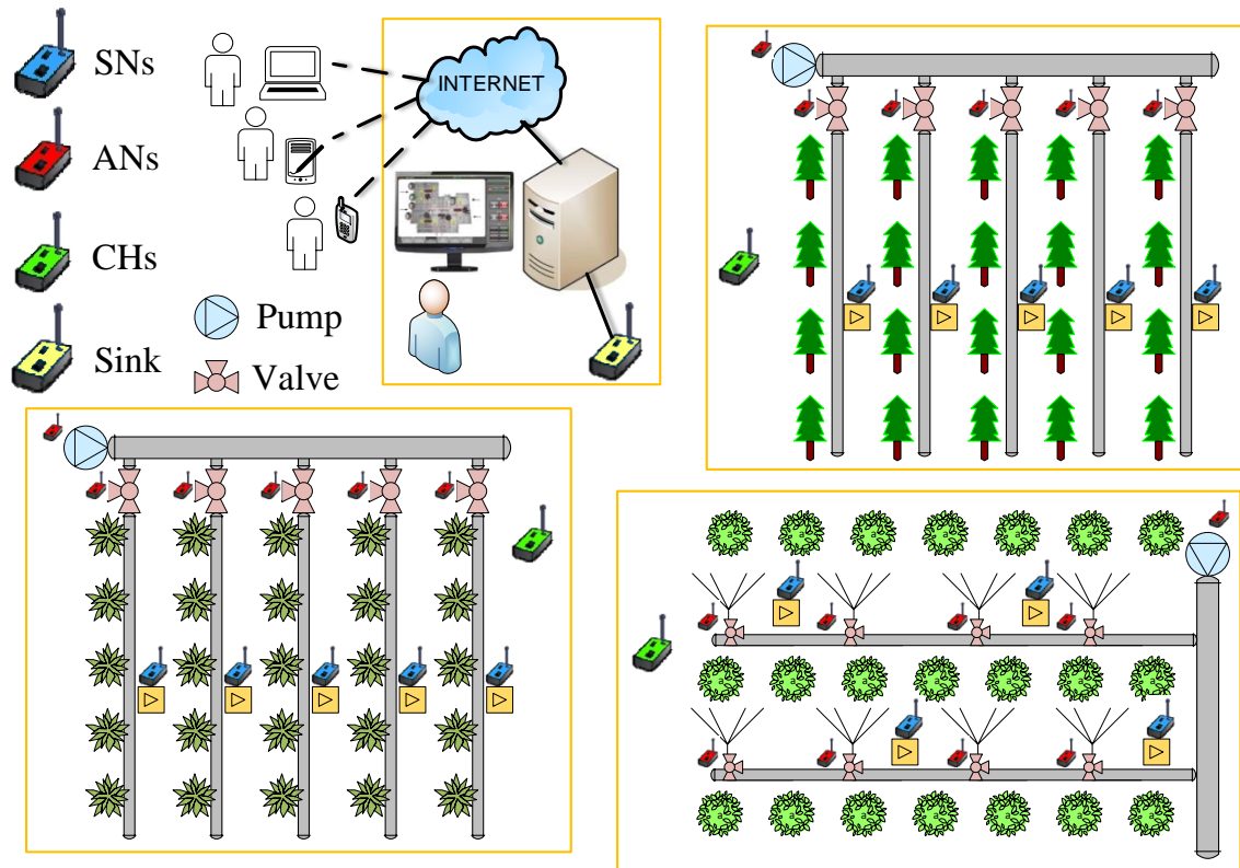
Figure 4. The system model of proposed network
