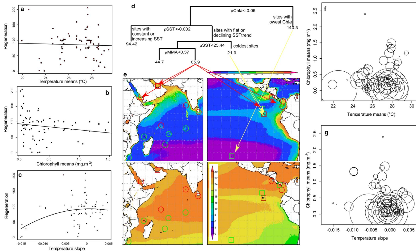
Figure 3 | Relationships of chl-a, SST and coral regeneration. (a,b) Linear relationships of regeneration with SST and chl- a means (c) quadratic relationship with the slope of a linear model of SST against time (~SST change 1981–2013). (d) Regression tree. Values at each branch are mean coral regeneration percentages in the group; \mu\text{chl-a} = mean chl- a , \rho\text{SST} = slope of SST over entire dataset, \mu\text{SST} = mean SST over entire dataset, \mu\text{MMA} = mean of monthly anomaly. Groups are indicated on (e) which are mean chl- a (1997–2010; in \text{mg.m}^{-3} ) and mean SST (2002–2010; in ^{\circ}\text{C} ) from MODIS Aqua (Circles = meta-analysis, squares = monitored sites, red = declining regeneration, green = steady/increasing regeneration.). (f) Bubble plots provide another view at SST, chl- a and regeneration. Coral regeneration as relative bubble size. Despite much scatter, regeneration decreases with increased chl- a levels (decreasing size of bubbles along y-axis).
