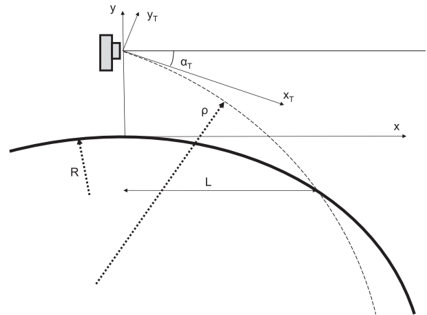
FIG. A2. Line-of-sight geometry with refraction.
