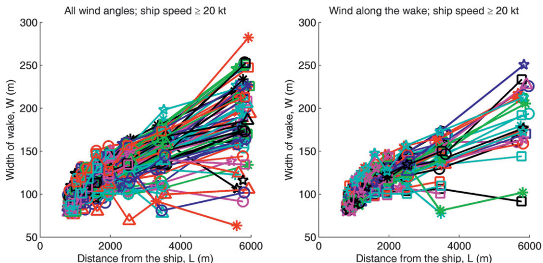
FIG. 11. Wake width vs distance plots for (left) all measured wakes and (right) relative wind direction within 30° of the ship track. Ship speed ranges from 20 to 24.4 kt.
