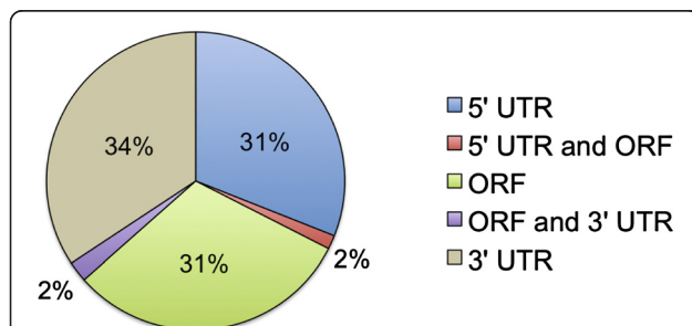
Figure 5 The proportion of white shark microsatellites within open reading frames (ORF) and untranslated regions (UTR). Red and purple sections show the proportions for a small number of microsatellites that straddled (i) the 5' end of the ORF and 5' UTR and (ii) the 3' end of the ORF and 3' UTR.
