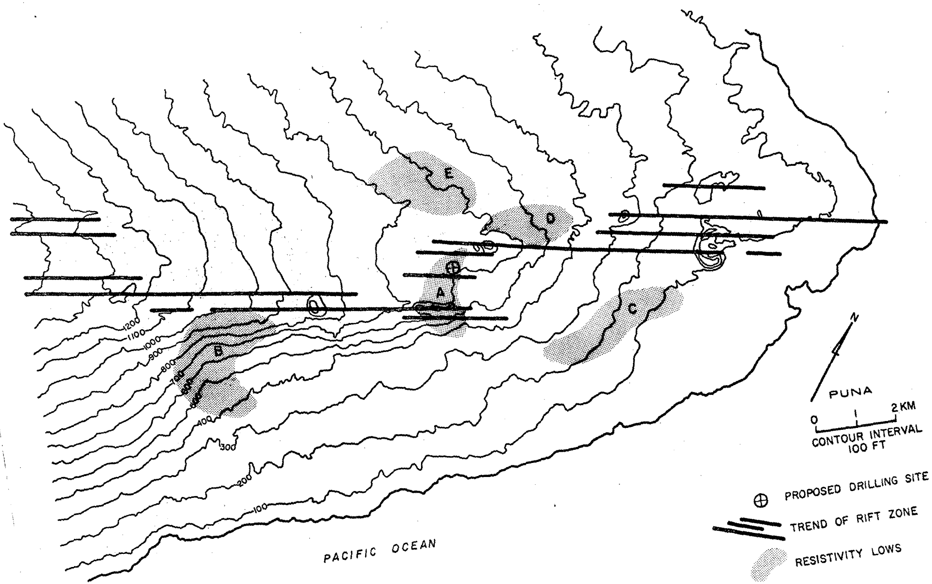
FIGURE 3. CONTOUR MAP OF PUNA AREA SHOWING TREND OF RIFT ZONE AND AREAS OF LOW ELECTRICAL RESISTIVITY
