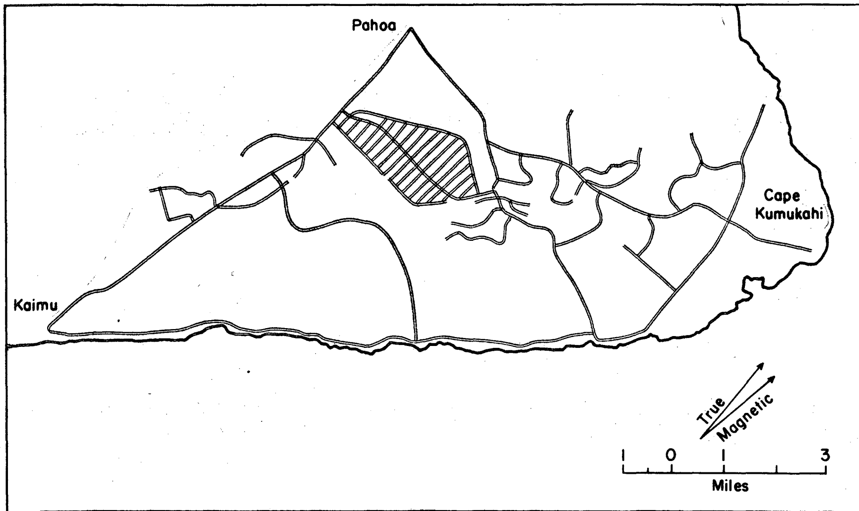
FIGURE 6. TRACKS OF MAGNETIC MEASUREMENTS IN PUNA AREA
