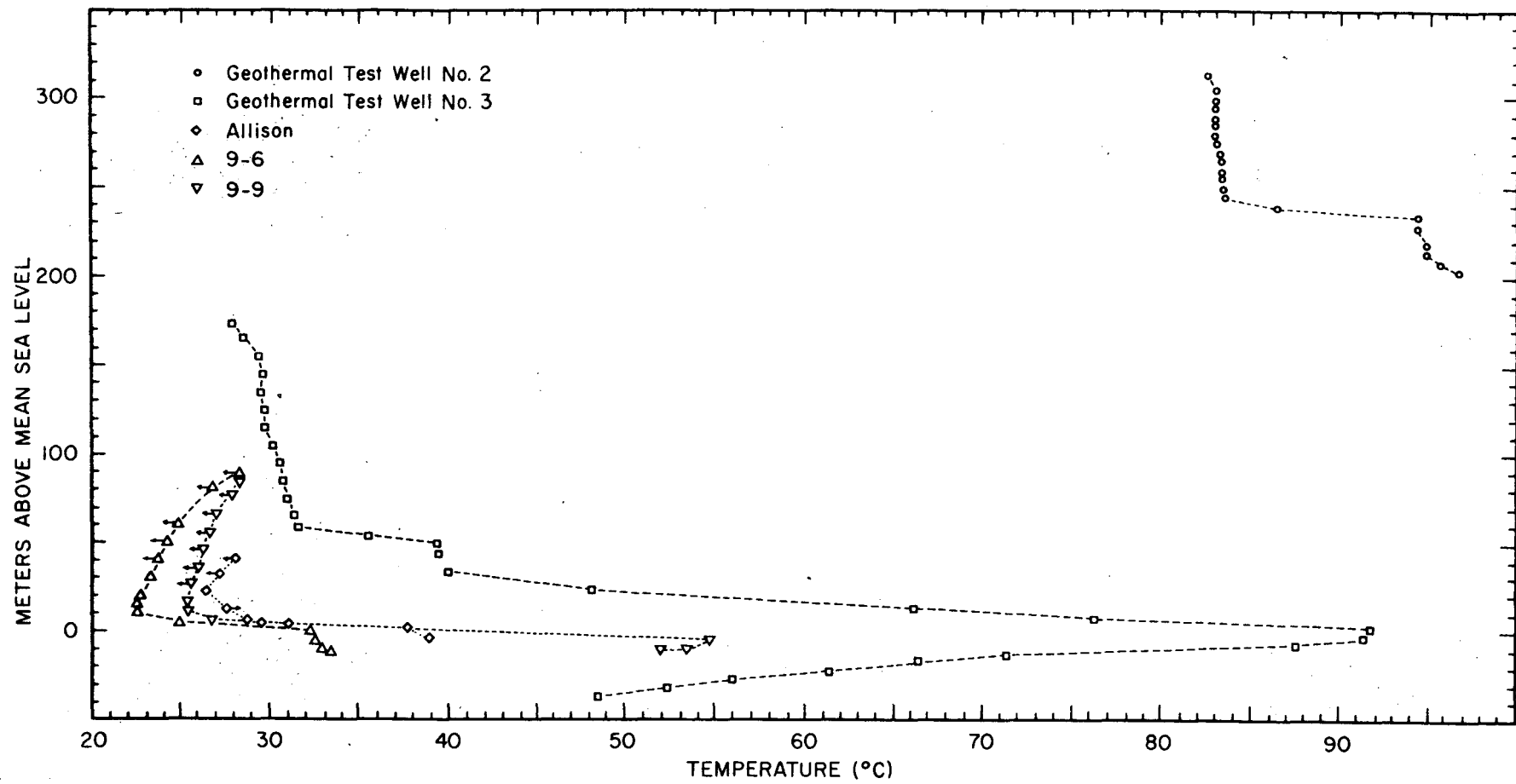
FIGURE 10. TEMPERATURE PROFILES OF FIVE WELLS IN PUNA, ISLAND OF HAWAII
