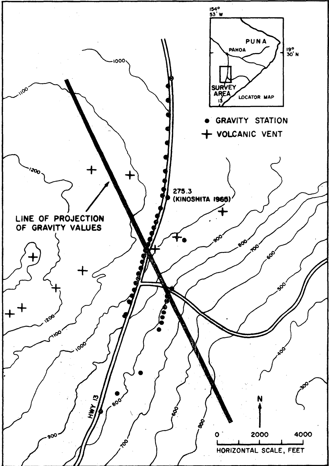
FIGURE 4. SURVEY AREA AND GRAVITY STATIONS
