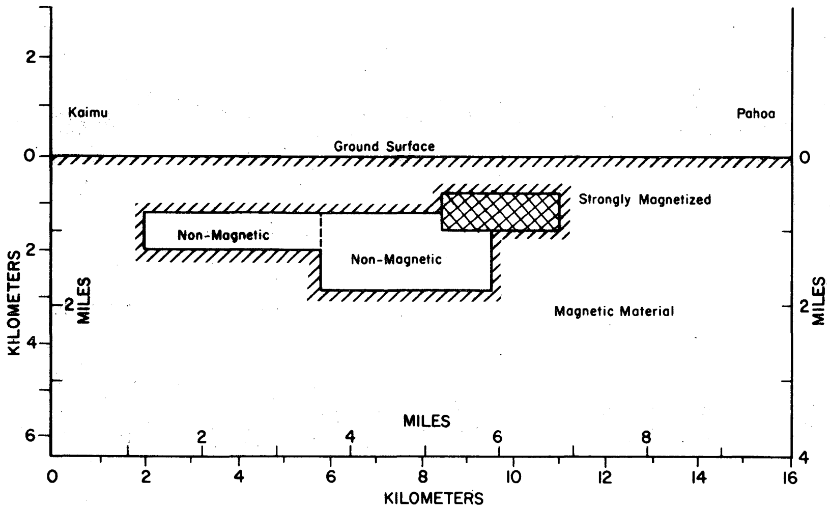
FIGURE 8. MAGNETIC ANOMALIES INFERRED FROM MAGNETIC PROFILE
