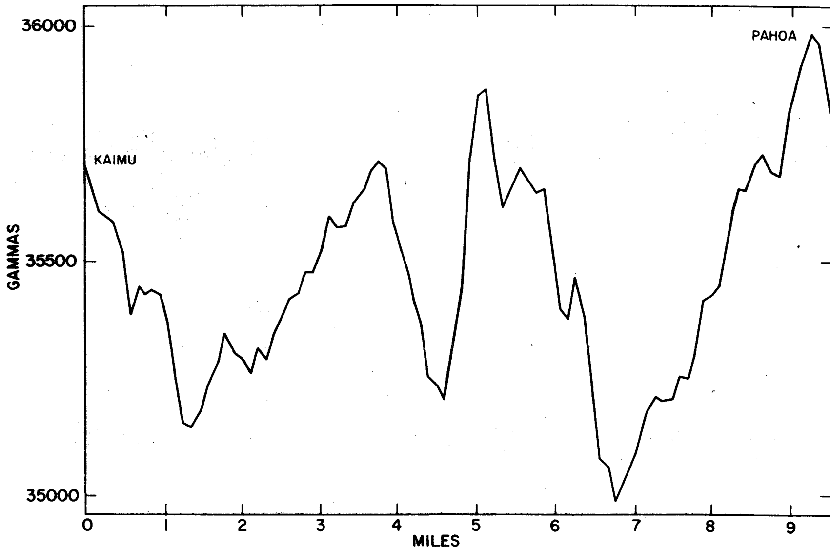
FIGURE 7. SPACE-FILTERED MAGNETIC PROFILE FROM KAIMU TO PAHOA
