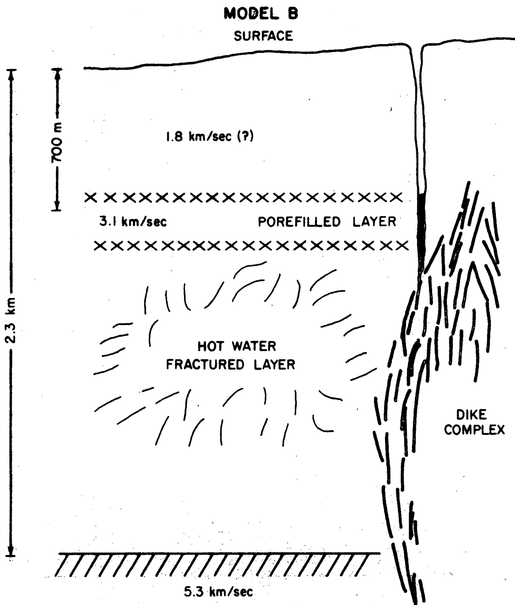
FIGURE 16. HYDROTHERMAL PROCESS OF AREA B. NOTE: THE MODEL IS VERY CONJECTURAL.
