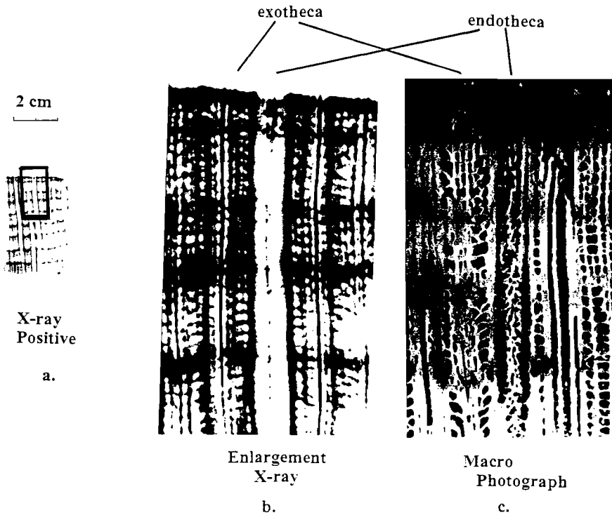
Fig. 8. a) X-radiograph positive print of 1.7 mm thick slab of Bahamas M. annularis . Black outlined area shows b) enlargement of X-radiograph with exothecal and endothecal areas included. c) macrophotograph enlarged to same scale as enlarged X-ray. HD bands appear restricted to exothecal area.
