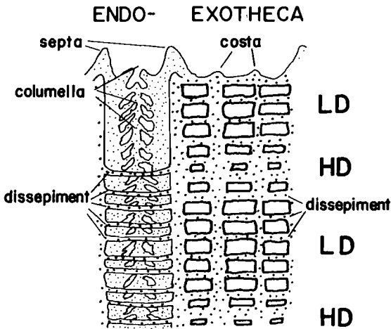
Fig. 9. Sketch of vertical section through M. annularis skeleton showing endotheal (corallite) and exotheal area. Stippled area indicates skeleton. Blank area indicates void space. High density (HD) and low density (LD) skeletal portions are indicated. HD banding results primarily from thickening of exothecal dissepiments and costa.
