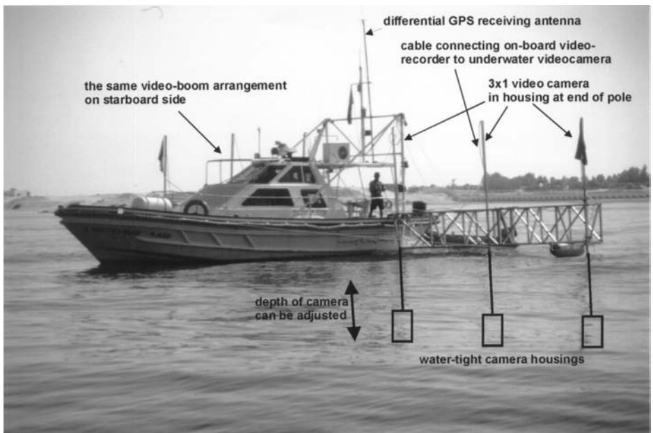
Figure 2. View of the survey vessel.
