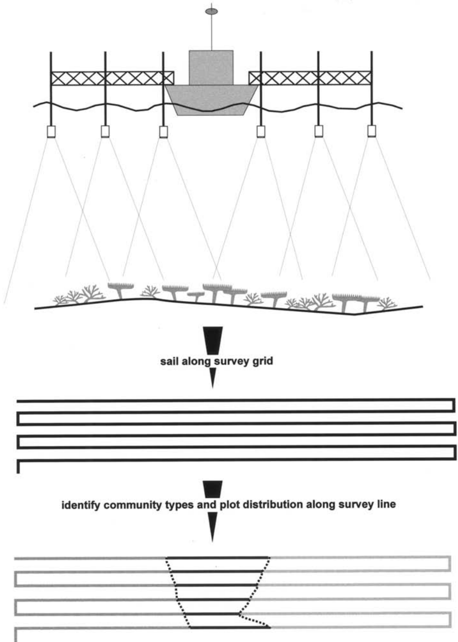
Figure 3. Overview sketch of the survey technology. The vessel is shown with downward facing video cameras. The fields of view overlap, providing a 24-m wide swath of continuous video coverage. The vessel sails along predetermined survey lines of 20 m spacing. Thus the entire surface area of the area of interest is recorded. Videos are then viewed and the spatial distribution (obtained by correlating video frame number with GPS data string) of previously determined bottom types marked along the survey lines printed on the chart. By connecting the contours between the adjacent survey lines, the spatial pattern becomes apparent.
