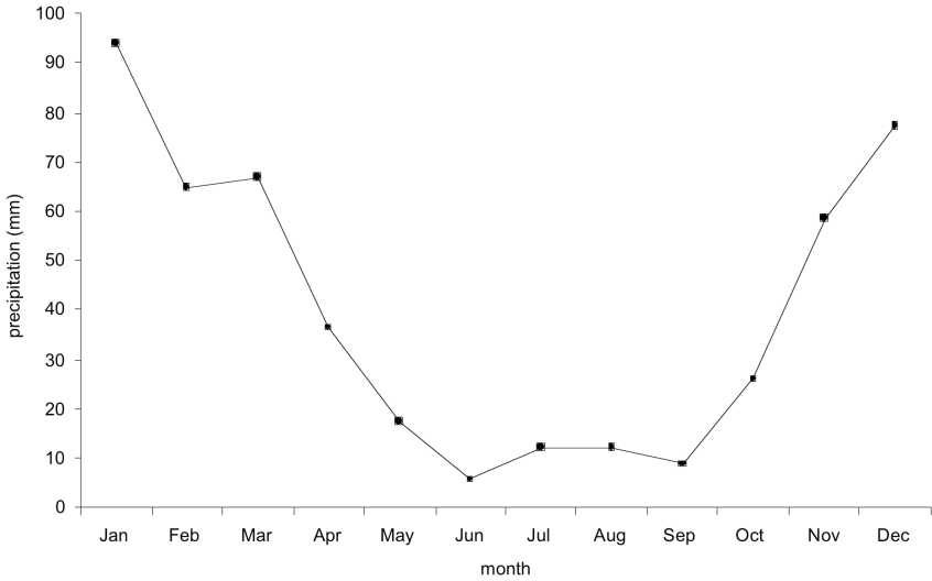
Figure 1. Mean monthly precipitation for Kahului, Maui (1954–2005).
