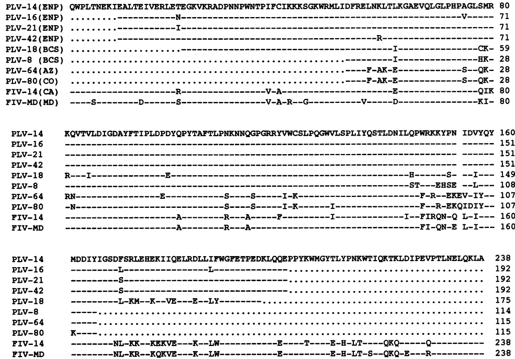
FIG. 2. Alignment of the predicted amino acid sequences of a conserved RT domain in the PLV and FIV pol genes (8, 28). Dashes below the PLV-14 sequence indicate identical amino acids. The open space is a gap introduced to maximize the alignment. Dots indicate sequences not obtainable with the available oligonucleotides used for PCR amplification. The geographical locations of virus isolation are indicated in parentheses. ENP, Everglades National Park; BCS, Big Cypress Swamp.
