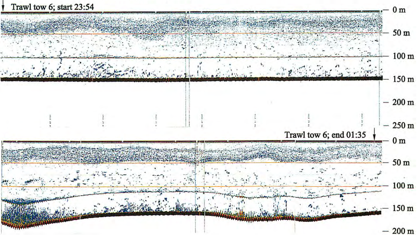
Fig. 11. Examples of echograms showing accumulations of epipelagic and epibenthic fishes. West of Fuerteventura; 11 April 1997.
