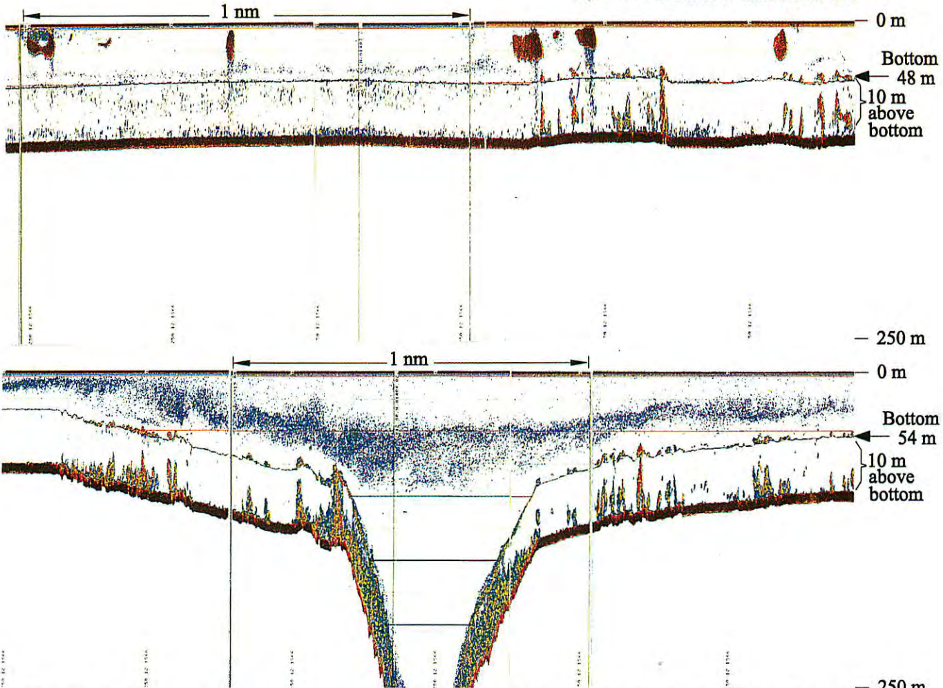
Fig. 11. Examples of echograms showing accumulations of epipelagic and epibenthic fishes. West of Fuerteventura; 11 April 1997.
