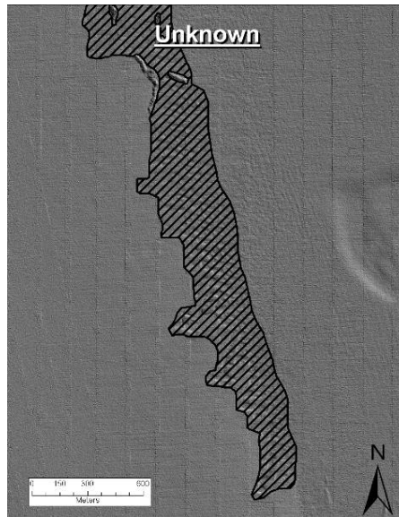
Figure 1.14: Illustration of bathymetric features interpreted as Unknown.
